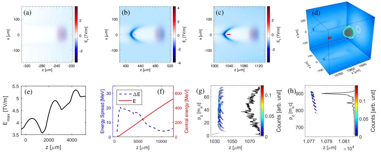
FIG. 3. (a-c) 2D slices of the laser, the plasma density and the injected electron beam. The red dots in (b) and (c) show the injected electrons. (d) 3D Snapshot at the optimal distance, where the blue color shows the plasma density projections to the 3 planes (multimedia view 1). (e) The laser peak electric field vs. z . (f) The energy and energy spread evolution of the injected beam. (g) and (h) show the (p_z, z) phase space distributions of injected electrons at the distances corresponding to the snapshot of (c) and (d), respectively. The black curves in (g) and (h) are the projections to the p_z axis (multimedia view 2).
