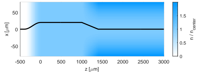
FIG. 2. Schematic diagram of the plasma profile in the simulations. The pseudo-color plot shows the distribution of the background plasma electrons, and the black solid line in the middle shows the longitudinal density profile of \text{C}^{4+} . The region from z = 0 to 1000 \mu\text{m} is uniform for both the background plasma and \text{C}^{4+} . The region from z = 1400 \mu\text{m} to infinite is a transversely parabolic channel without \text{C}^{4+} . The region from z = -400 to 0 \mu\text{m} is a transition from vacuum to the plasma, and the region from z = 1000 to 1400 \mu\text{m} is a transition from the uniform region to the channel. The axial plasma density in the channel is the same as the density of the uniform region.
