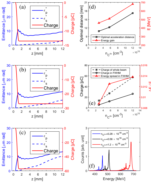
FIG. 4. Plots showing the electron beam qualities in three cases. The evolutions of the trapped electron beam charge (red curves) and the normalized transverse emittance (blue curves) with n_{C^{4+}} = 0.28, 0.56 and 1.2 \times 10^{16} \text{ cm}^{-3} are illustrated in (a), (b), and (c) respectively, where the solid and dashed blue curves are the emittances in the directions paralleled to and perpendicular to the laser polarization direction, respectively. (d) The optimal acceleration distance and the energy gain at this distance vs. n_{C^{4+}} . (e) The final charge (absolute number) of the whole beam, the charge within FWHM respect to the peak energy in the spectrum, and the relative energy spread in FWHM at optimal acceleration distance vs. n_{C^{4+}} . (f) The energy spectra at the optimal acceleration distance for the three cases.
