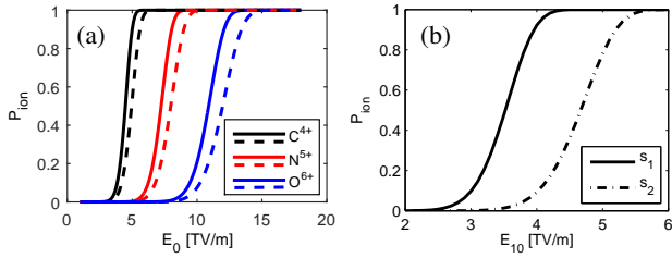
FIG. 1. Ionization probability after one laser cycle vs. laser electric field amplitude for different situations predicted by the ADK model. (a) The laser is either with the wavelength of 2.4 \mu\text{m} (solid lines) or with 0.8 \mu\text{m} (dash lines). The black/red/blue colors represent the cases of \text{C}^{4+} , \text{N}^{5+} and \text{O}^{6+} , whose L-shells have already been stripped off by laser pre-pulses. (b) The laser is square-wave-like bichromatic with wavelengths of 2.4 \mu\text{m} and 0.8 \mu\text{m} , and the ionization object is \text{C}^{4+} . The solid line shows the ionization probability after one laser cycle when the combined electric field takes the form of E_{10} \left[ \cos(\omega t) + \frac{1}{3} \cos(3\omega t) \right] , and the dash-dot line shows that when it takes the form of E_{10} \left[ \sin(\omega t) + \frac{1}{3} \sin(3\omega t) \right] .
