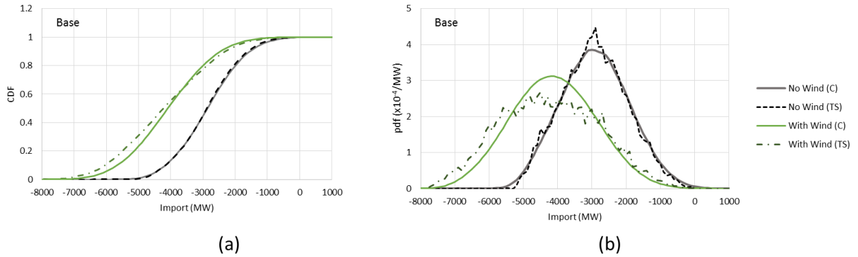
Figure 5: (a) cumulative and (b) density plots of convolved and time series estimations (denoted C and TS respectively) of boundary import requirements for the base case scenario with and without wind.
