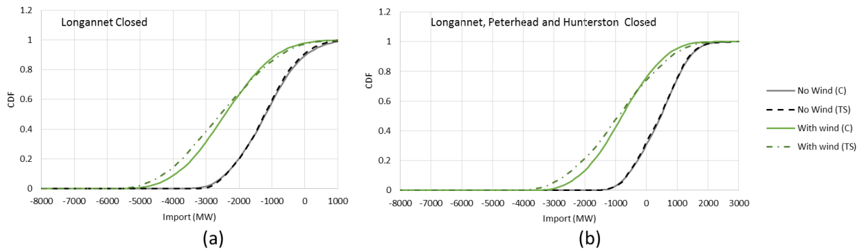
Figure 6: cumulative distribution for 'Longannet Closed' and 'Low Conventional' cases estimated by convolved and time series analysis (denoted C and TS respectively) with and without the existing wind fleet.
