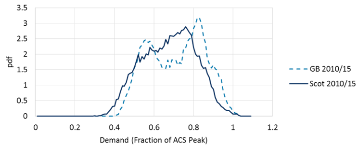
Figure 4: Distribution of winter demand for GB and Scotland 2010 – 2015 as a fraction of weather corrected peak demand.
