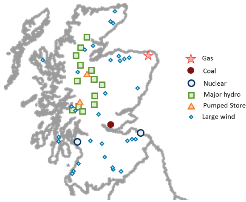
Figure 1: location of main generation plant within Scotland.
