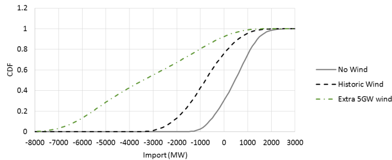
Figure 7: The impact of wind capacity on boundary requirements for the 'Low Conventional' and 'High Wind Future' scenarios.
