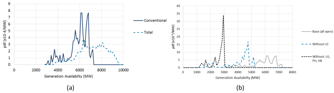
Figure 3: (a) Winter historic generation availability in Scotland 2013 – 15. ‘Conventional’ includes coal, nuclear, gas, hydro and pumped storage; ‘Total’ includes all conventional plus wind. (b) Availability representing conventional generation in the main scenarios.
