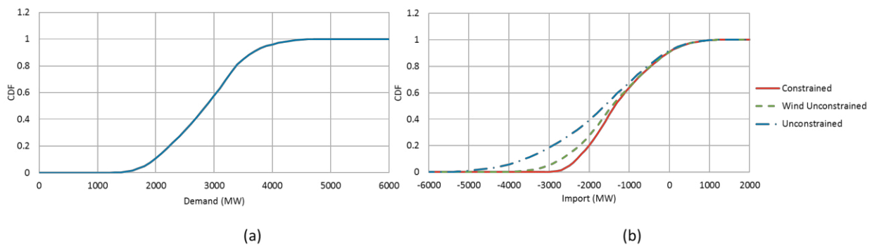
Figure 2: (a) cumulative distribution for demand in 2015; and (b) cumulative distribution for import to Scotland (negative values represent exports) estimated from demand, nominated generation and constraint actions.
