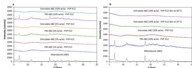
Figure 2. Diffractograms of (a) ABZ – PVP K12 formulations at time zero and (b) ABZ – PVP K12 at 10/90 % (w/w) after 6 months storage
