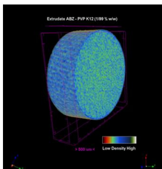
Figure 1. Micro-CT image of ABZ – PVP K12 extruded material at 1/99 % (w/w)
