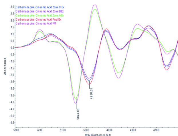
Scheme 5 Second derivative of in-line NIR spectra in the mixing zones (A, B, and C) of extruded cocrystals in a twin – screw extruder and the physical mixture. Reproduced from Ref. 103 with permission from The Royal Society of Chemistry.
