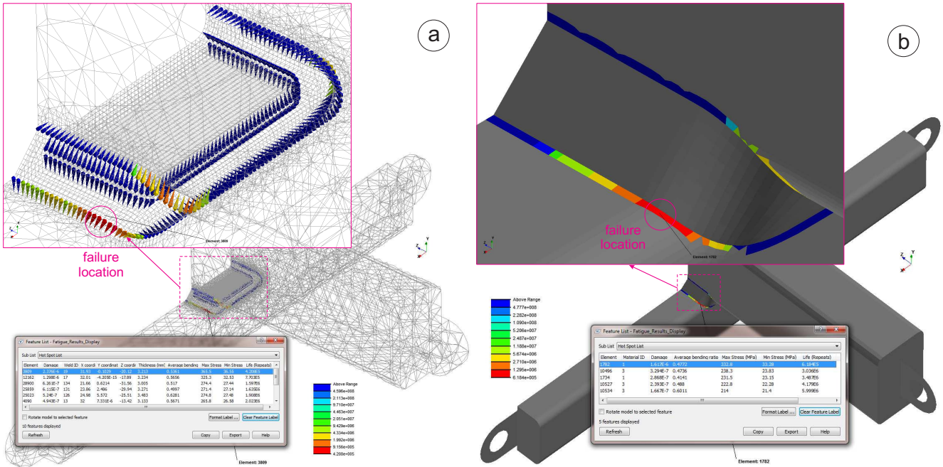
Fig. 1: Result of fatigue life predictions (cycles) for 75x50x3 RHS to 50x50x3 SHS connection for (a) solid and (b) shell FE-models.
