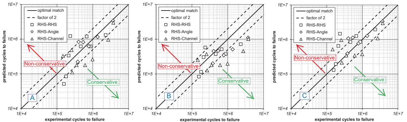
Fig. 2: Comparison of the observed and predicted cycles to failure using shell elements for: a) S-N curves for SM490B steel welds; b) new generic S-N curves in nCode DesignLife c) old generic S-N curves in nCode FE-Fatigue.
