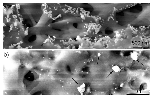
Figure 3. SEM images of CA membranes; a) Membrane top showing nanoparticle building blocks interacting with the membrane; b) Membrane bottom showing large electron-dense particles (indicated by arrows).
