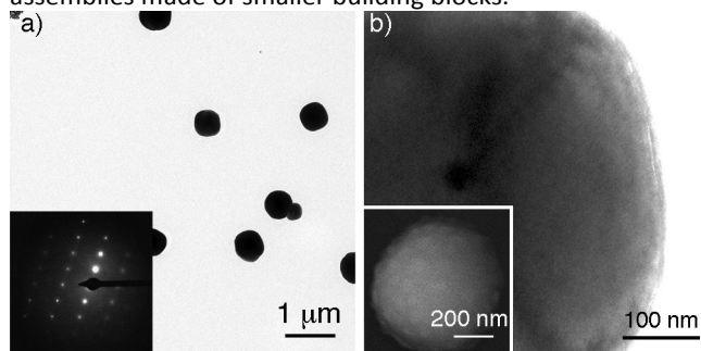
Figure 1. Gold supraparticles found after filtering gold nanoparticles through a CA membrane; a) TEM images of the supraparticles; Inset: SAED pattern of a single supraparticle; b) High-magnification TEM image of a supraparticle; Inset: SEM image of a supraparticle
