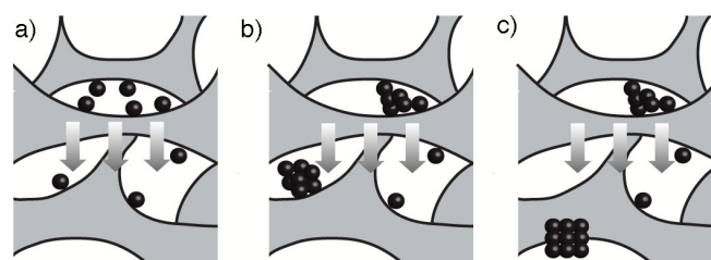
Figure 4. Schematic representation of the main steps involved in the formation of gold supraparticles upon filtration through a CA membrane; a) gold nanoparticles interact with the CA membrane and reduce the pore size; b) nanoparticle aggregates are formed; c) as they flow through the filter the nanoparticles in the aggregates realign and generate crystallographically aligned supraparticles at the bottom of the filter. The arrows indicate the direction of the solution flow.
