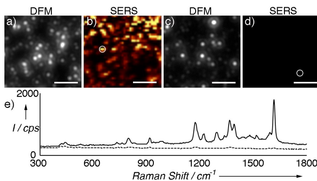
Figure 2. SERS analysis of supraparticles modified with malachite green isothiocyanate; a), b) Correlated dark-field microscopy (DFM) image and SERS map of supraparticles adsorbed onto a glass slide; c), d) DFM image and SERS map of nanoparticle building blocks; e) Representative SERS spectra of supraparticles (solid line, highlighted with a circle in (b)) or nanoparticle building blocks (dotted line, circle in (d)). SERS images were generated from analysis of the peak intensity at \sim 1172 \text{ cm}^{-1} with respect to the background signal with the brightest points corresponding to intensities >300 \text{ counts/s} (cps). See also Figure S7 in ESI and experimental details below. Scale bars: 5 \mu\text{m} .
