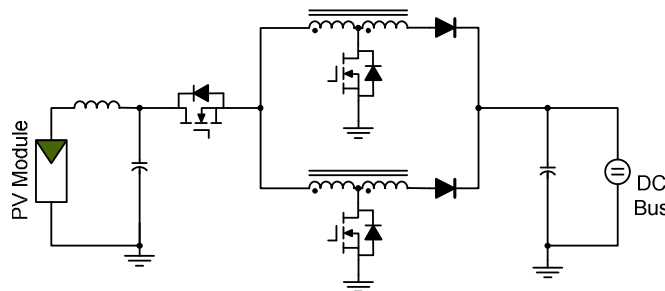
Fig. 12. Circuit of Module-Integrated-Parallel Converter proposed by eIQ energy Inc.
