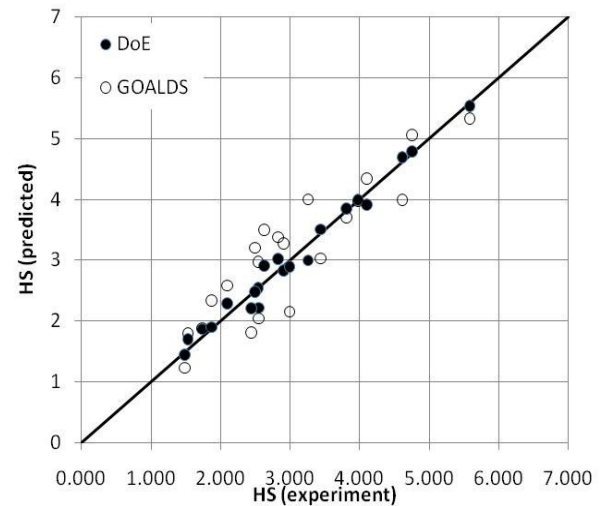
Figure 2: Comparison between predicted and experimental survivalability results, using SOLAS 2009 (HARDER - Top) and (GOALDS - bottom) s-factor formulations.
