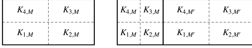
Fig. 4 A macro element M \in \mathcal{P}_0 (left) and set \omega_\gamma (right) with cells K_{i,M} \in \mathcal{P} .
