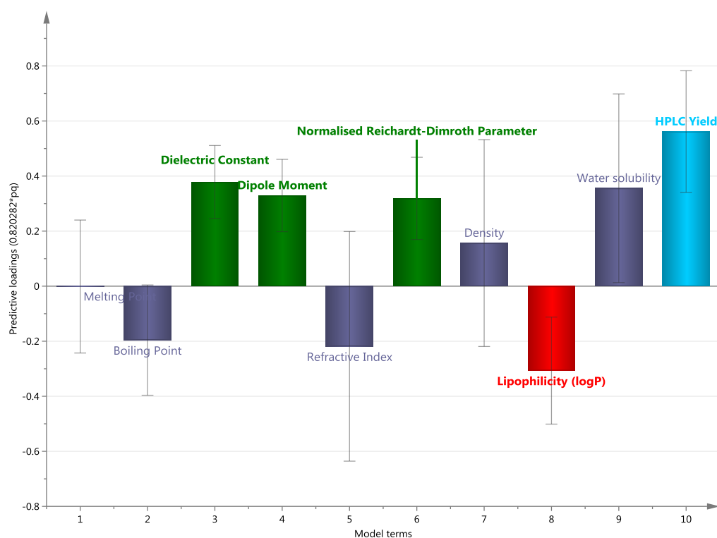
Figure 3: OPLS regression model
