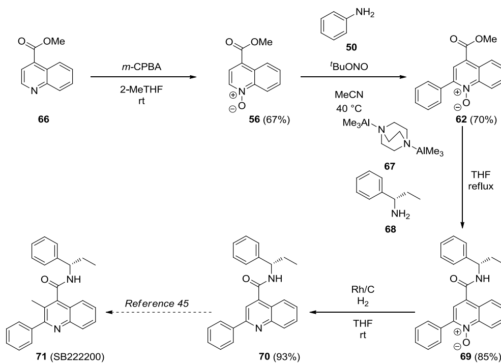
Figure 12: Formal synthesis of SB222200
