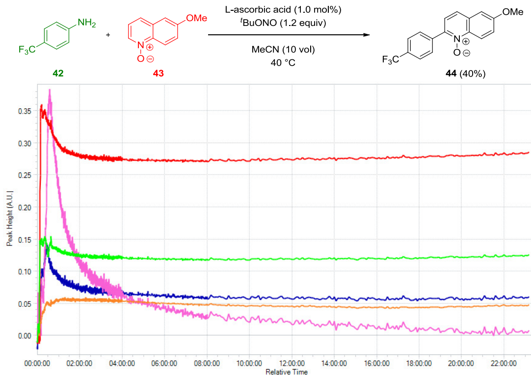
Figure 8: Wavenumbers monitoring and potential intermediate identification
