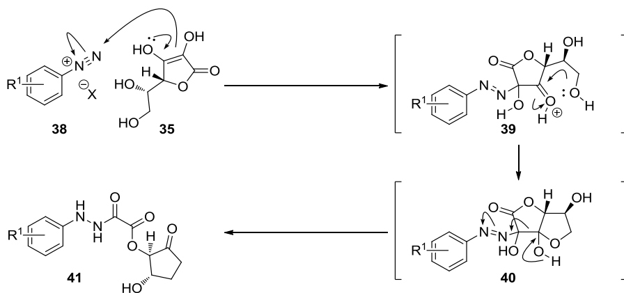
Figure 7: Japp-Klingemann rearrangement for hydrazine formation 40
