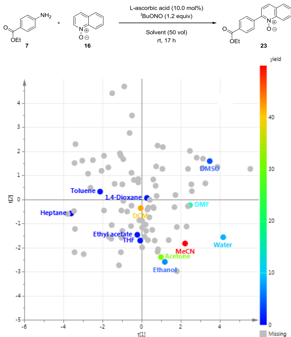
Figure 2: PCA solvent model
