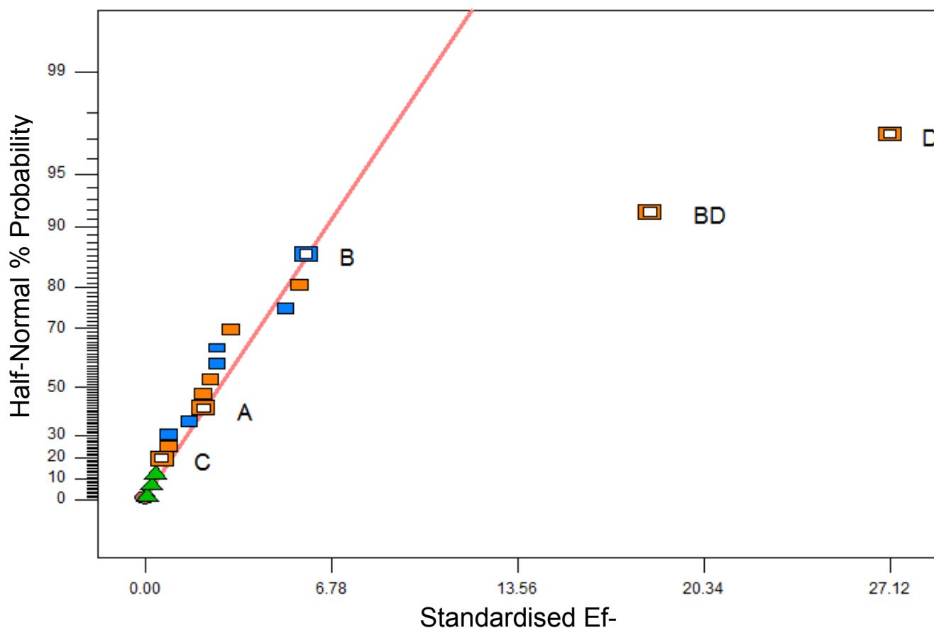
Figure 4: Half-normal plot using HPLC yield as response
