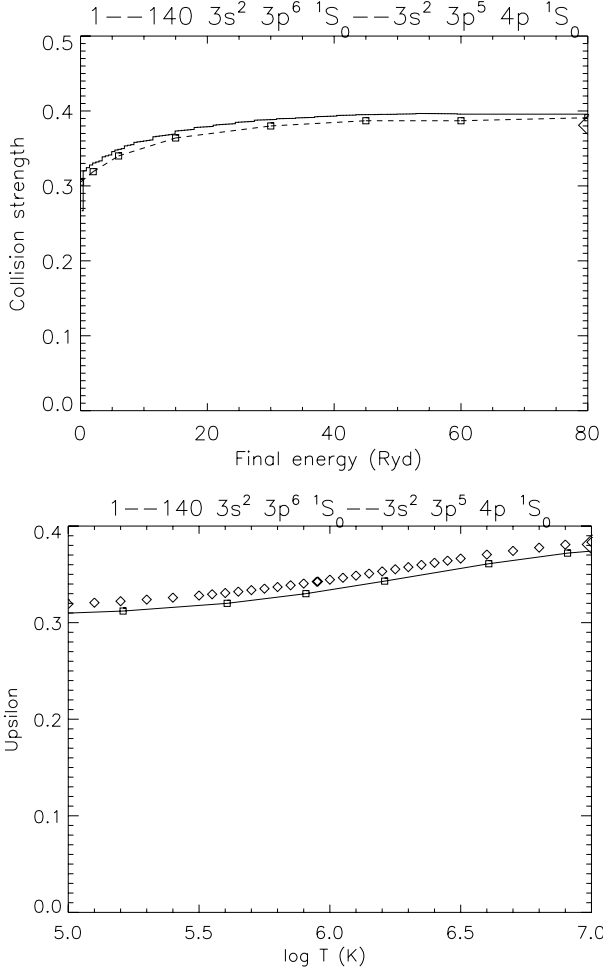
Fig. 2. Top: collision strength for the 3s^2 3p^6 \ ^1S_0 - 3s^2 3p^5 4p \ ^1S_0 transition of Fe IX. Squares with dashed line from present results. Histogram from Storey et al. (2002). Bottom: thermally averaged collision strength for the 3s^2 3p^6 \ ^1S_0 - 3s^2 3p^5 4p \ ^1S_0 transition. Solid line with squares from present results. Diamonds from Storey et al. (2002).
