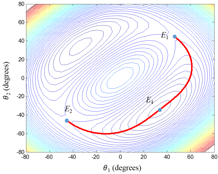
Figure 13. Uncontrolled heteroclinic connection between E_1 and E_2 in the original untransformed coordinate axes (\theta_1, \theta_2) .
