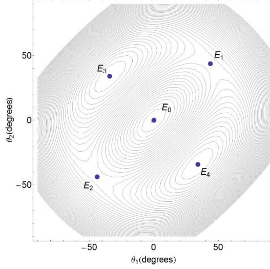
Figure 9. Potential V(\boldsymbol{\theta}, \boldsymbol{\kappa}) and equilibria (3 unstable equilibria E_0 , E_1 and E_2 , and 2 stable equilibria E_3 and E_4 ).
