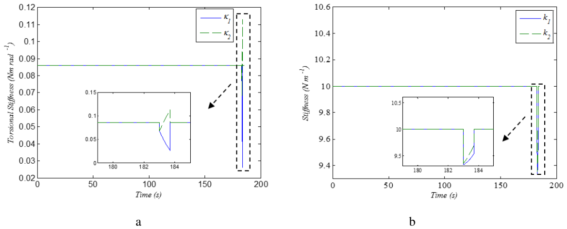
Figure 22. Controls actuated at the end of the transition. (a) torsional spring stiffness, (b) axial spring stiffness.
