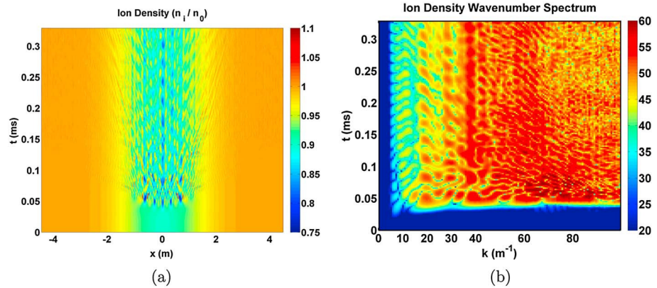
Figure 2. Time evolution of the normalized ion density n_i/n_0 in (a) space and (b) wave number space.
