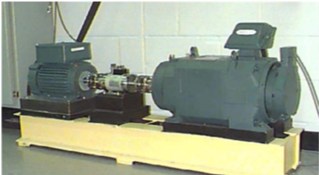
Figure 5: The bearing test rig [65]
