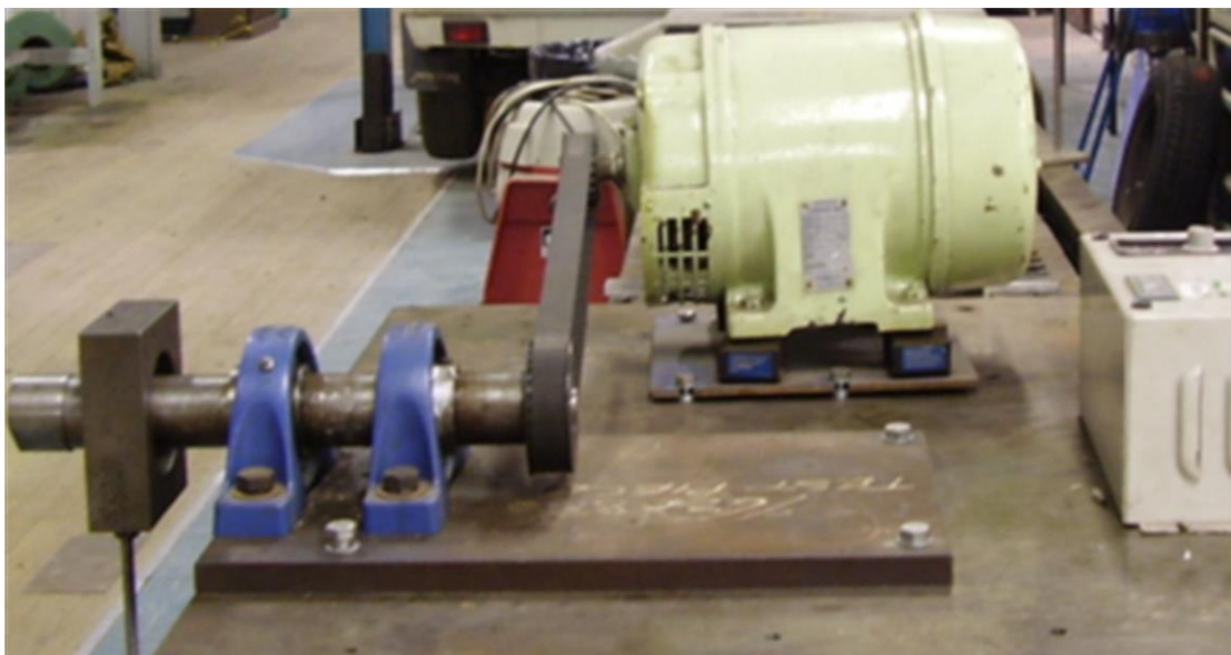
Figure 6: Bearing test rig at Strathclyde University
