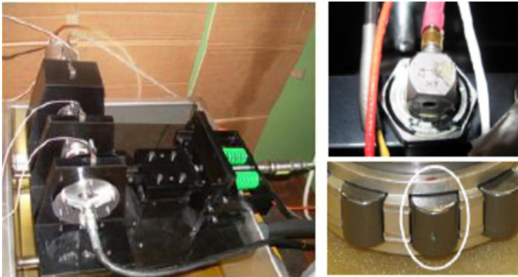
Figure 7: DIRG test rig, the triaxial accelerometers (X, Y, Z) and the damaged roller used in the tests [56]
