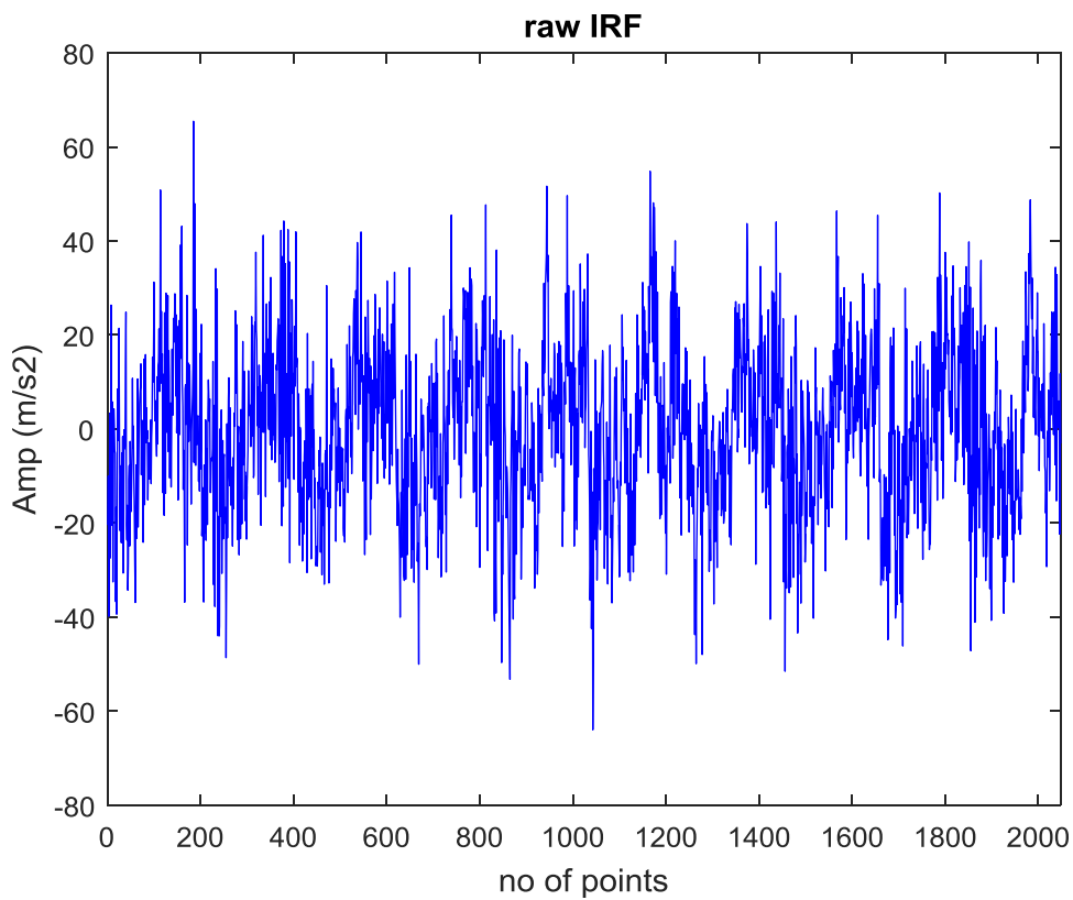
Figure 8: A signal from data set 3, a bearing with inner race fault
