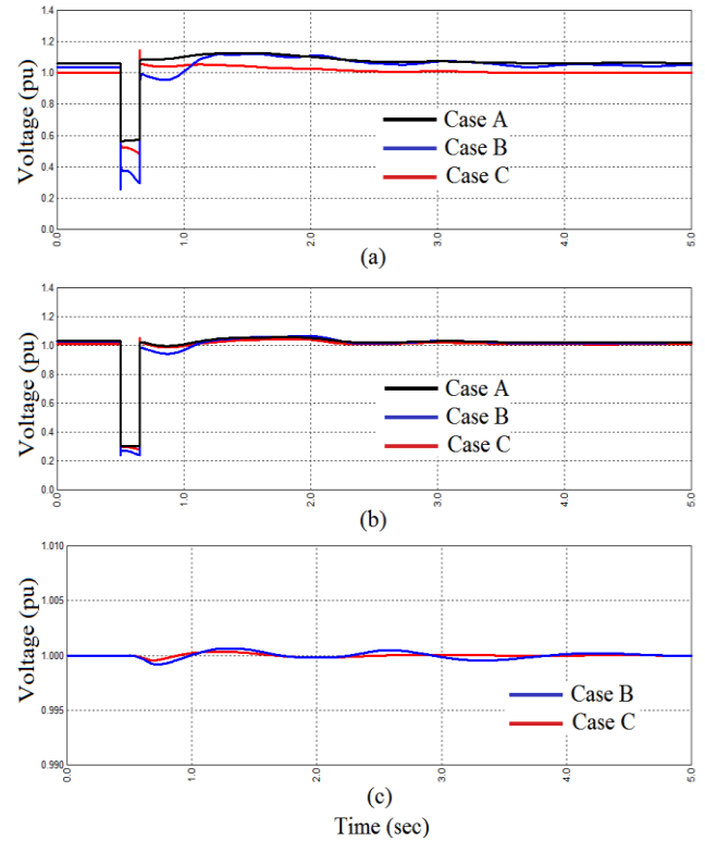
Figure 7. Transient responses of the test system voltage, (a) voltage of the critical bus 16, (b) terminal voltage of the onshore side converter and G_7 (bus 36) and (c) terminal voltage of the offshore side converter for each case.
