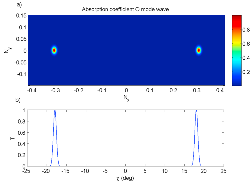
Figure 3. (a) Absorption coefficient for the O mode as a function of the normalized wave vector components N_x and N_y , and (b) of the incidence angle \chi at \phi = 0 . The absorption is significant for angles of incidence only within a few degrees near the Spitzze angle \chi_S = 17.95^\circ at \phi = 0 .
