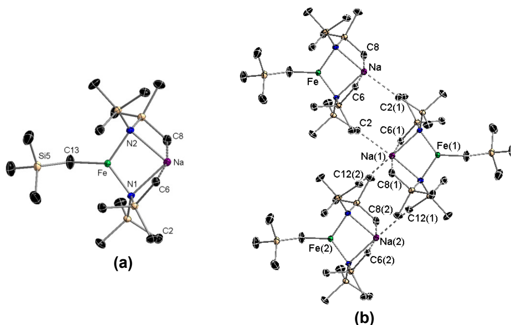
Figure 2: (a) Asymmetric unit of [\{\text{NaFe}(\text{HMDS})_2(\text{CH}_2\text{SiMe}_3)\}_\infty] ( 2 ). Hydrogen atoms omitted for clarity. Thermal ellipsoids displayed at 50% probability level. Selected bond distances (Å) and angles (°): Fe-N1 2.0308(17), Fe-N2 2.0306(17), Fe-C13 2.051(2), Na-C6 2.7013(21), Na-C8 2.7275(21), Fe \cdots Na 3.0401(9), Na-N1 2.4804(19), Na-N2 2.4702(19), N1-Fe-N2 107.96(7), N1-Fe-C13 129.08(10), N2-Fe-C13 121.83(10), Na-N1-Fe 84.11(6), Na-N2-Fe 84.38(6), Na-Fe-C13 165.55(7), N1-Na-N2 83.14(6). (b) Section of polymeric chain showing intermolecular and intramolecular Na-Me contacts Na(1)-C2 2.838(4) Å, Na(1)-C12(2) 3.041(2) Å.
