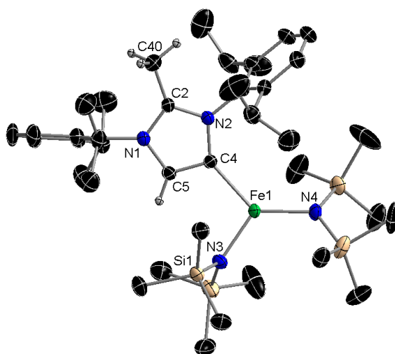
Figure 6 - Molecular structure of complex 6 with selective atom labelling. Hydrogen atoms minor disorder components in \text{SiMe}_3 groups omitted for clarity. Thermal ellipsoids displayed at 50% probability level. Selected bond distances ( \text{\AA} ) and angles ( ^\circ ): Fe-C4 2.113(2), Fe-N3 1.9732(19), Fe-N4 1.9459(19), C2-N1 1.330(4), C2-N2 1.341(3), C2-C40 1.491(3); C4-Fe-N3 104.02(8), C4-Fe-N4 132.84(8), N3-Fe-N4 123.14(8), Fe-C4-N2 140.30(16), C40-C2-N1 125.3(2), C40-C2-N2 126.9(2), N1-C2-N2 107.46(19)
