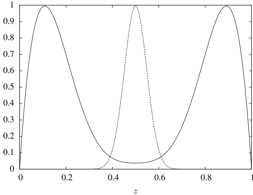
Figure 1: Scaled \psi(0.5, z) (solid line) and \psi(5, z) (dashed line) versus z
