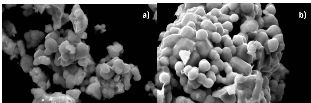
Figure S5: SEM images of the Al-doped LLZ sample prepared via microwave-assisted (a) and conventional (b) solid-state approaches. The mean particle size for the microwave-assisted prepared samples is 1.5 \pm 0.4 \mu\text{m} while for the sample prepared via conventional solid-state approach displays an average particle size slightly bigger of 2.3 \pm 0.9 \mu\text{m} .
