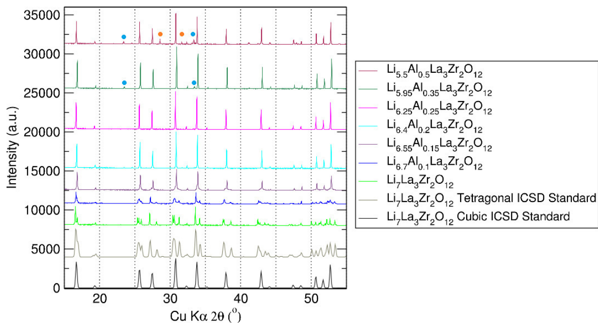
Figure S3: PXRd patterns for the LLZ garnet with increasing Al concentration from bottom to top. Reference patterns are included for the cubic ( I\bar{a}3d ) and tetragonal ( I4_1/acd ) symmetries. [1,2] Blue dots denote \text{LaAlO}_3 impurity and orange dots denote \text{La}_2\text{Zr}_2\text{O}_7 impurity.
