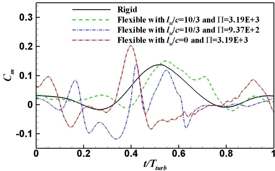
Figure 31 Instantaneous moment coefficient at \lambda=5.5
