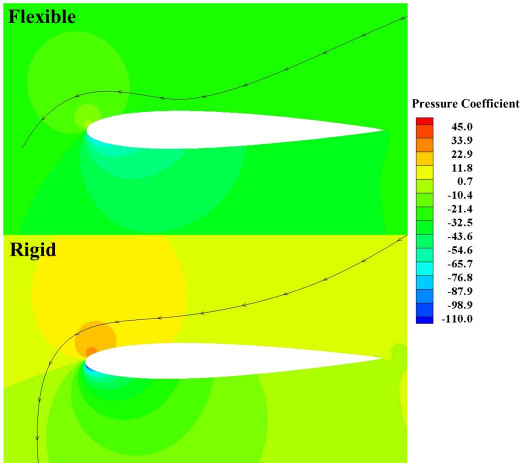
(c) Pressure distribution around blade at t/T_{\text{turb}}=5/8 .
