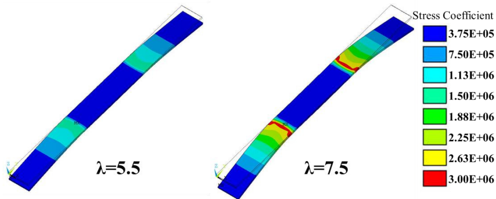
Figure 16 Contour of stress distribution over the blade under the largest external load condition for the flexible blade for different tip speed ratio with l_{st}/c = 10/3 and \Pi = 3.19 \times 10^3 viewing from the inner side of blade
