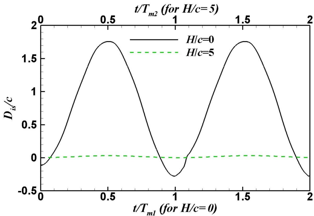
(a) Instantaneous non-dimensionalized displacement
