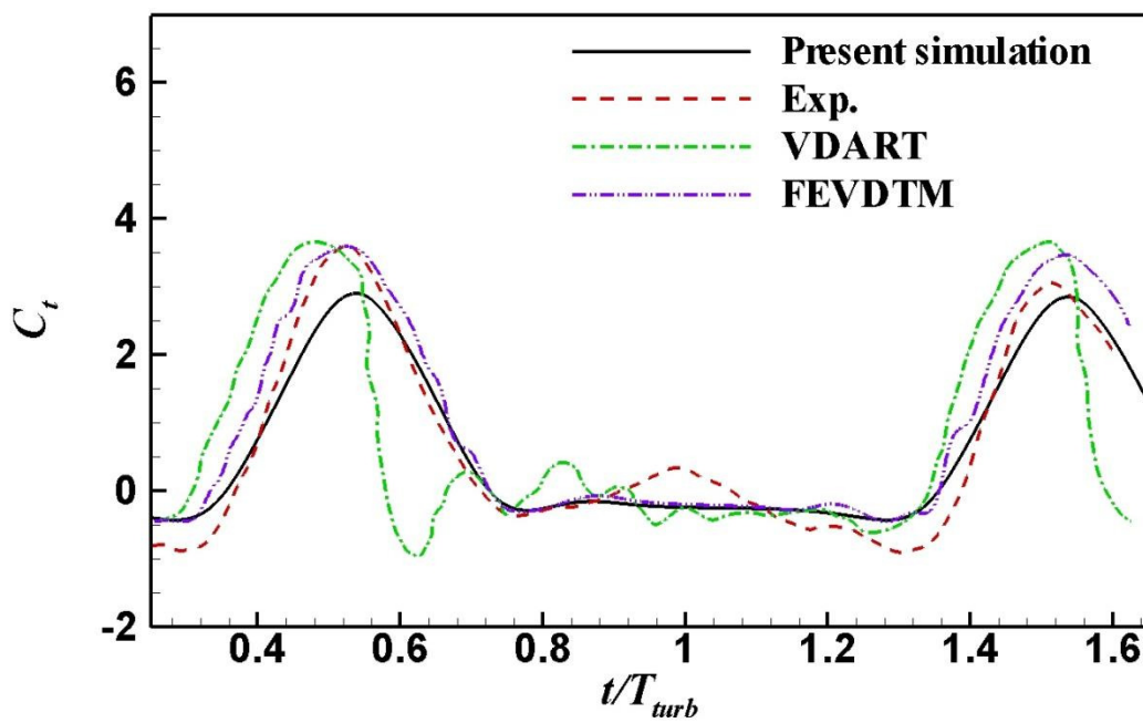
(b) Instantaneous thrust coefficient
