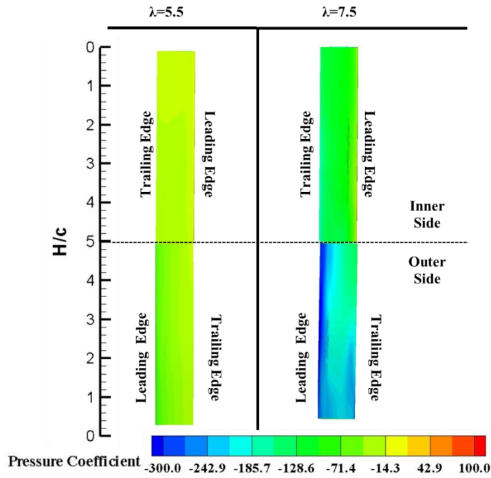
Figure 20 Pressure distribution at t/T_{\text{turb}}=5/8 for different tip speed ratios with l_{st}/c=10/3 and \Pi = 3.19 \times 10^3
