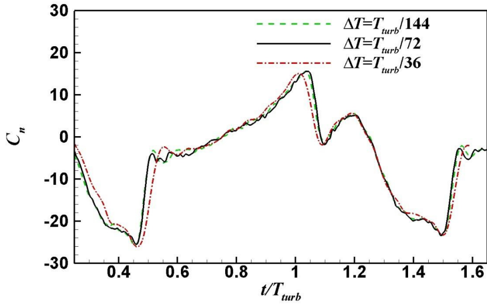
Figure 7 Sensitivity study of time step size
