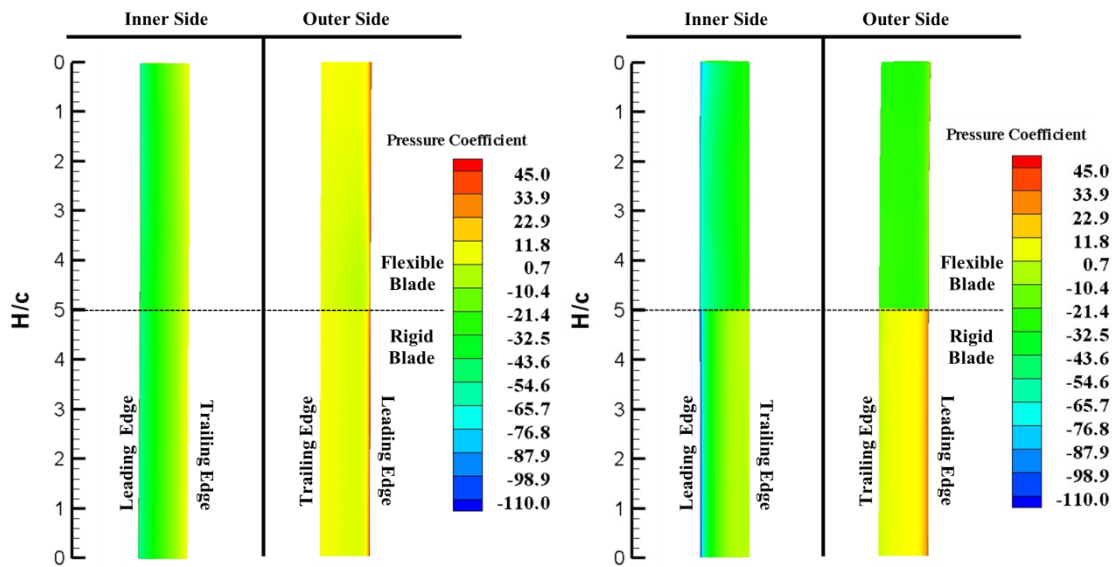
Figure 17 Blade bend-twist motion and pressure distribution for different time instants with l_{st}/c=10/3 , \Pi = 3.19 \times 10^3 and \lambda=5.5
