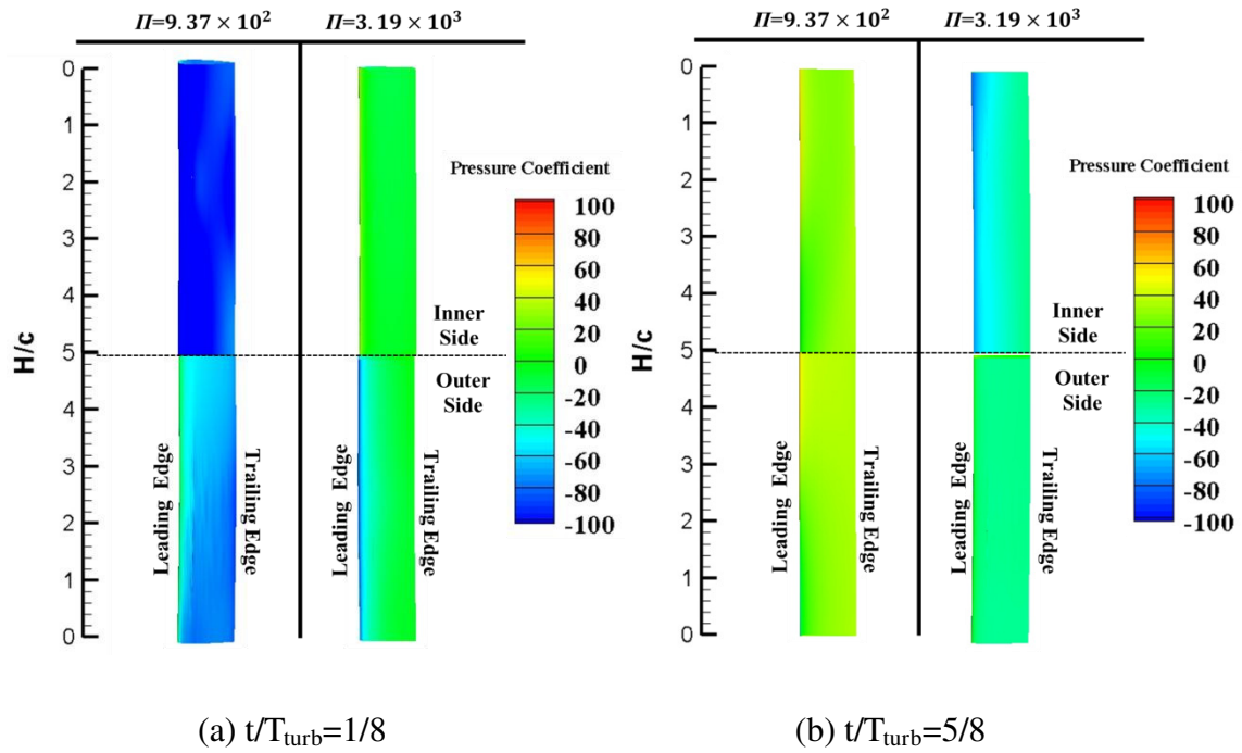
Figure 25 Pressure distribution at (a) t/T_{\text{turb}}=1/8 and (b) t/T_{\text{turb}}=5/8 with l_{st}/c=10/3 , \lambda=5.5 and \Pi = 9.37 \times 10^2 compared with \Pi = 3.19 \times 10^3
