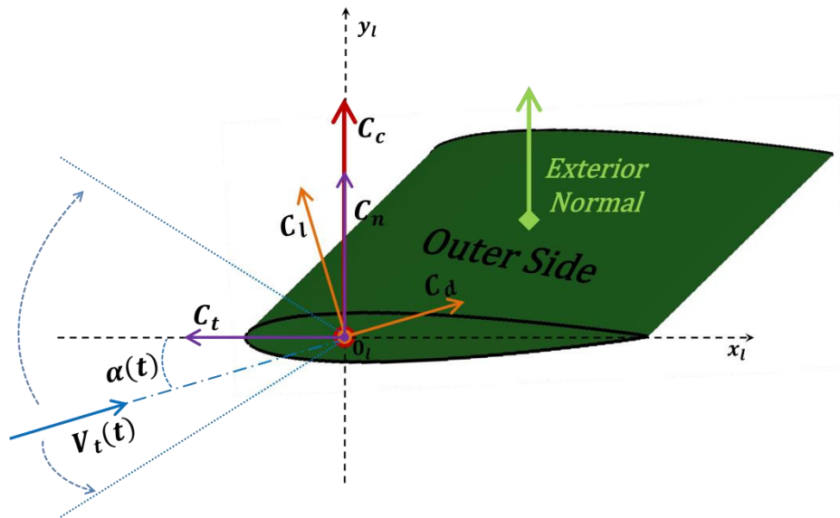
Figure 2 Sketch of turbine blade forces, resultant velocity and angle of attack under local body fitted coordinate x_1, o_1, y_1
