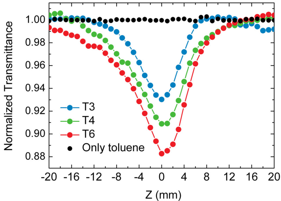
Figure 2. Open aperture z-scan measurement of the nonlinear absorption cross-section. Normalized transmittance of the Gaussian laser beam (800 nm, 120 fs and 1kHz repetition rate) through a 1 mm quartz cuvette containing 10 mM of T3, T4, T6 and only toluene, measured by the open aperture z-scan technique.
