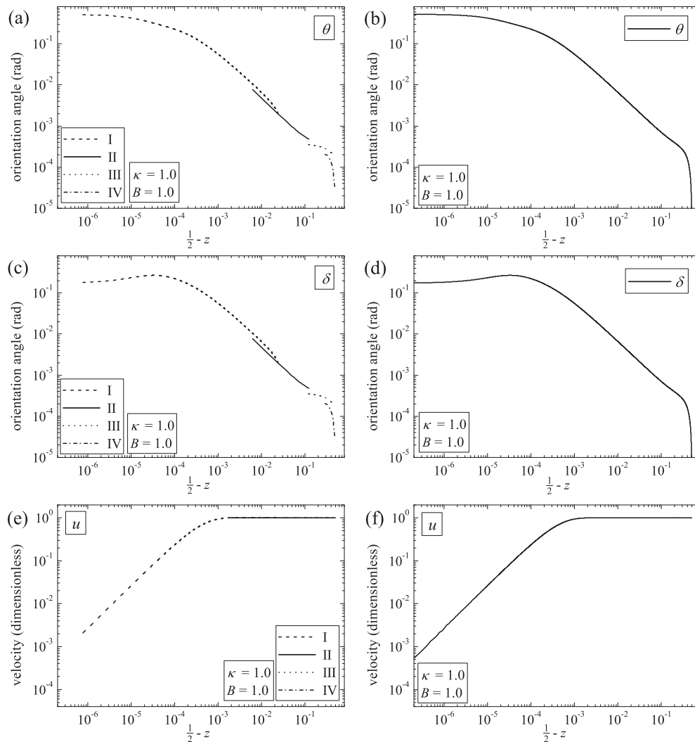
FIG. 10. The figures on the left are derived from the asymptotic results discussed in the text for the four key layer regions identified in Figure 9, whereas those on the right are from direct numerical computations, all taken as functions of \frac{1}{2} - z and for the fixed parameter values \kappa = 1 and B = 1 . (a) and (b) show \theta , (c) and (d) show \delta , and (e) and (f) show u .
