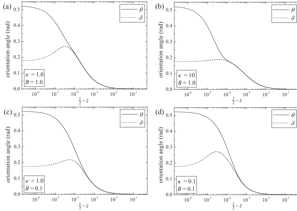
FIG. 11. Numerically derived solutions to the dynamic problem for \theta and \delta as functions of \frac{1}{2} - z with \lambda_p = 10^{-16} . (a) \kappa = 1, B = 1 ; (b) \kappa = 10, B = 1 ; (c) \kappa = 1, B = 0.1 ; (d) \kappa = 0.1, B = 0.1 .
