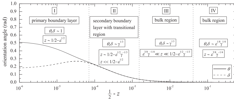
FIG. 9. A schematic description of the four key regions (separated by dotted vertical lines) that identify the main boundary layer phenomena of the dynamic problem discussed in the text.
