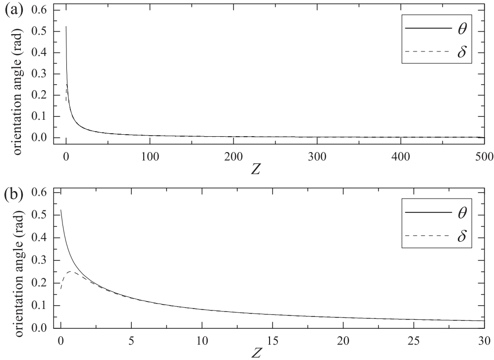
FIG. 6. The dependence of \theta and \delta upon Z (static case). (a) The domain 0 \leq Z \leq 500 . (b) A restriction of the result in (a) to the domain 0 \leq Z \leq 30 , which emphasizes the boundary layer effects.
