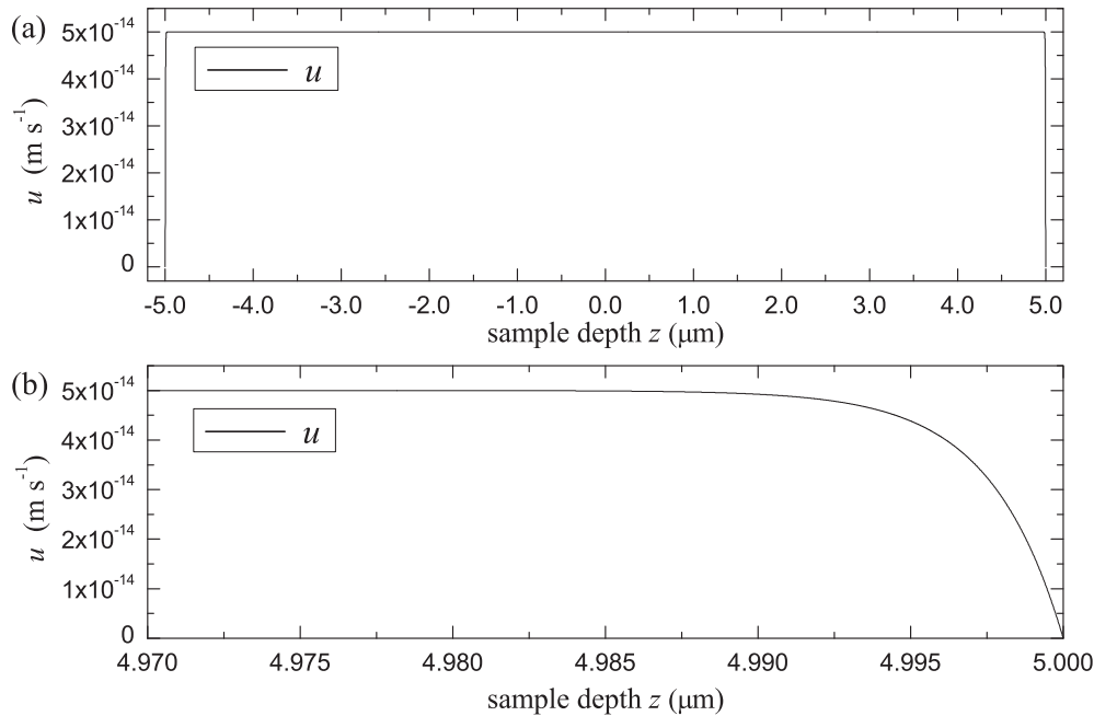
FIG. 4. Plots of the solution for u given by (3.20), using the material parameters from Table 1. (a) The velocity profile for u across the sample -d/2 \leq z \leq d/2 . (b) The boundary layer near z = d/2 ; a similar effect occurs at z = -d/2 , by symmetry. The boundary layer can be estimated via (3.24) and, in this example, is of the order of L_1 = \sqrt{\eta\lambda} \sim 2.4 \text{ nm} .
