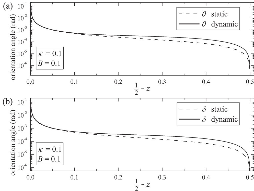
FIG. 12. A comparison of the results for \theta and \delta for the steady state dynamic problem in Figure 11(d) with the results for the static problem derived in [32, Figure 10(d)].
