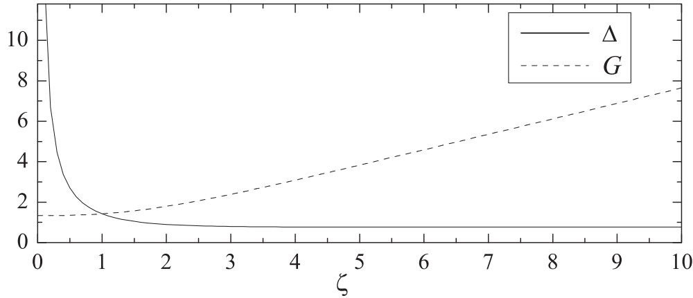
FIG. 8. The dependence of \Delta and G on \zeta .
