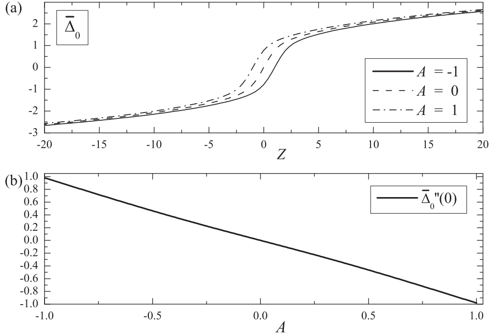
FIG. 7. (a) The dependence of \bar{\Delta}_0 upon Z for A = -1, 0 , and 1 . (b) The dependence of \bar{\Delta}_0''(0) upon A .
