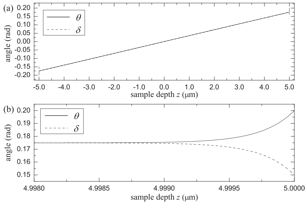
FIG. 3. Plots of the exact solutions for \theta and \delta provided by (3.18) and (3.19) using the material parameter values stated in Table 1 when \theta_0 = 0.2 rad and \delta_0 = 0.15 rad. (a) Solutions over the full sample depth -d/2 \leq z \leq d/2 . The profile is virtually linear away from the boundaries, as explained in the text. (b) The occurrence of a boundary layer is evident near the boundary at z = d/2 , with a similar effect at z = -d/2 , by symmetry. The boundary layer is roughly of the order of L_2 = \sqrt{K_1^a/2B_1} \sim 0.25 nm.
