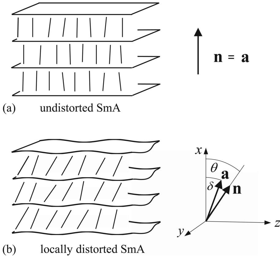
FIG. 1. (a) A schematic diagram of locally arranged planar layers of SmA liquid crystal. In an undistorted configuration in the bulk, away from any boundary influences, the layers prefer to be equidistant and the local layer normal \mathbf{a} coincides with the director \mathbf{n} . (b) The layer and director alignments may be perturbed from their preferred undistorted orientations, in which case \mathbf{a} and \mathbf{n} need no longer coincide. The orientation angles \theta and \delta , for \mathbf{n} and \mathbf{a} , respectively, are measured relative to the direction of the undistorted layer normal.
