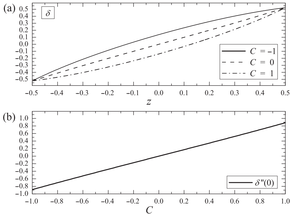
FIG. 13. (a) The dependence of \delta on z for C = -1, 0, 1 . (b) The dependence of \delta''(0) on C .
