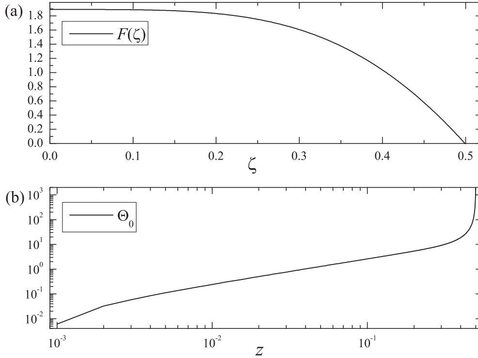
FIG. 5. (a) The dependence of F upon \zeta . (b) \Theta_0 as a function of z (static case).
