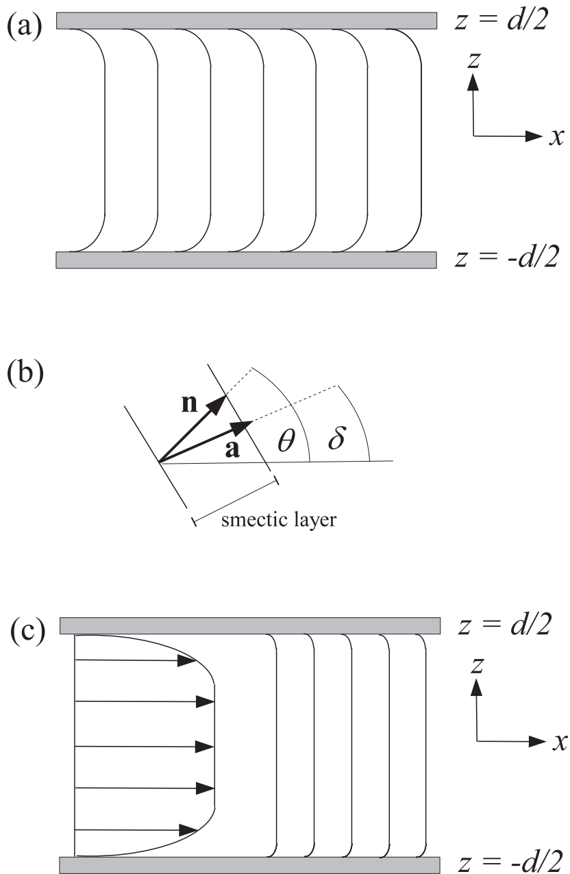
FIG. 2. (a) A schematic illustration of the anticipated alignment of the SmA layers in a steady state situation when there is a pressure-driven flow in the x -direction. The liquid crystal is placed between two parallel fixed boundary plates located at z = \pm d/2 and the sample is assumed to be uniformly aligned in the y -direction. Boundary layers are expected to occur which will have a consequent effect upon the orientation of the SmA layers near the boundaries. (b) The local orientation angles of \mathbf{n} and \mathbf{a} in relation to the local smectic layer profile are described by \theta(z) and \delta(z) , respectively, measured relative to the horizontal x -axis. (c) A diagram of the anticipated plug-like permeation flow normal to the smectic layers mentioned by de Gennes [11]. The velocity profile is expected to be relatively flat except near the boundary walls.
