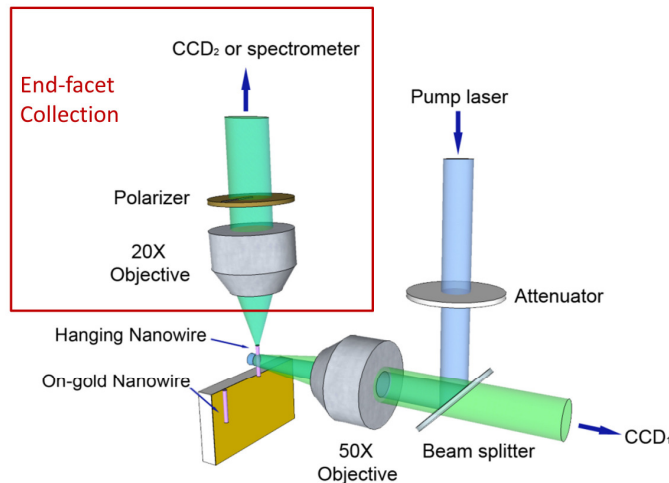
Fig. 1. Schematic of the two-arm micro-PL setup. In the pump arm (right), an incident laser beam pumps the GaN nanowires from the side. In the collection arm (left), the objective is aligned along the nanowire axis so that its polarization can be measured accurately.
