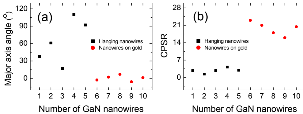
Fig. 4. Statistics of (a) polarization major axes and (b) CPSRs from 10 nanowires with similar geometry (5 hanging nanowires and 5 gold substrate nanowires).
