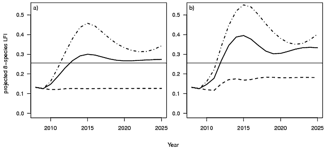
Fig. 4. Time-series projections of the modelled eight-species LFI under two cod recruitment scenarios a) pre-settlement model mortality parameters unaltered from the baseline, and b) a 'gadoid outburst' with increased survival of pre-settlement cod. Each panel contains three fishing scenarios – 2008 fishing mortalities (dashed lines), F_{MSY} (solid lines), and the cessation of fishing (dot-dashed lines). The horizontal line indicates the eight-species LFI target value (0.26).
