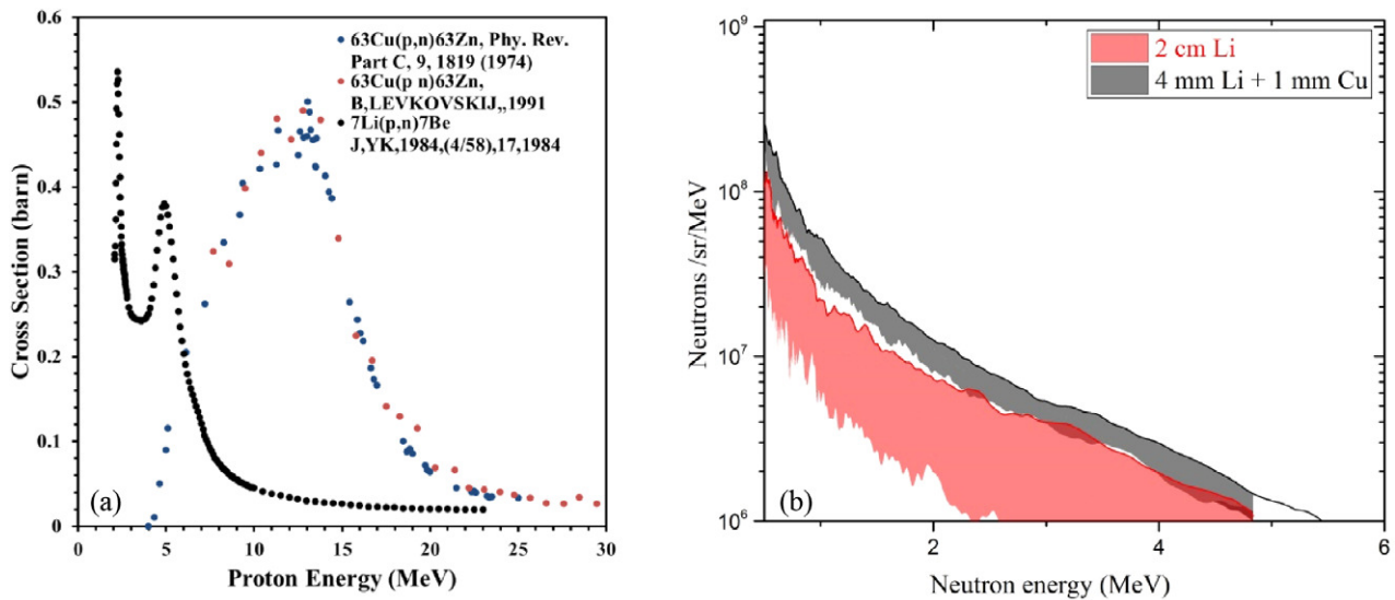
Figure 3. (a) Neutron generation cross sections as a function of proton energies impinging on lithium and copper and (b) measured neutron spectra for the two convertor designs.
