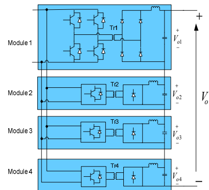
Fig.2 IPOS converter system topology
