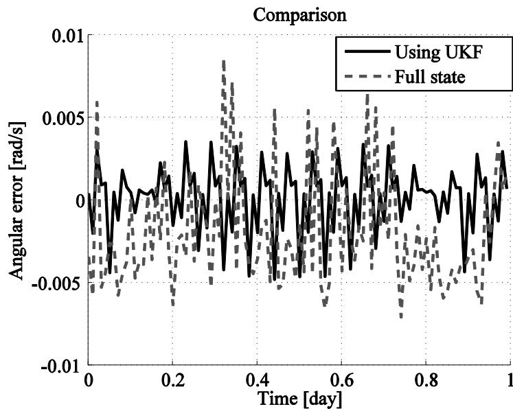
Figure 10. Angular error estimation using full state optical flow and optical flow with Kalman filter.
