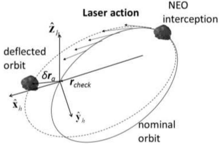
Figure 18. Asteroid's proximal motion.
