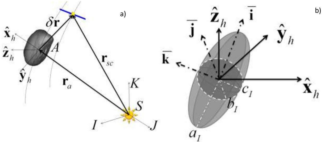
Figure 3. (a) Definition of the inertial and Hill's reference frames; (b) definition of the asteroid's body fixed reference frame.
