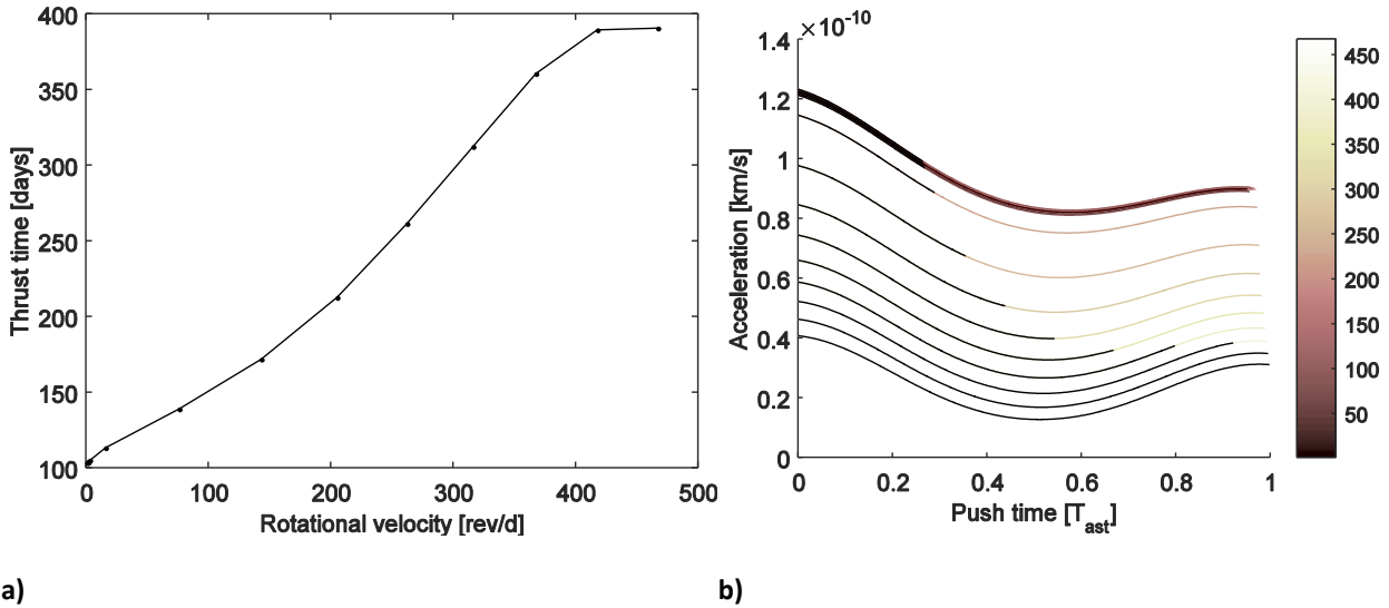
Figure 17. a) Thrust time to achieve the target delta-velocity change as function of the initial rotational velocity of the asteroid. b) Actual acceleration onto the asteroid as function of time with different initial rotational velocities of the asteroid (colour bar). The black portion of the lines represents the time needed to achieve the target change in velocity of 1 m/s.
