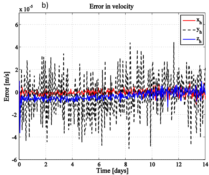
Figure 11. Spacecraft Control -Estimated position (a) and velocity error (b).
