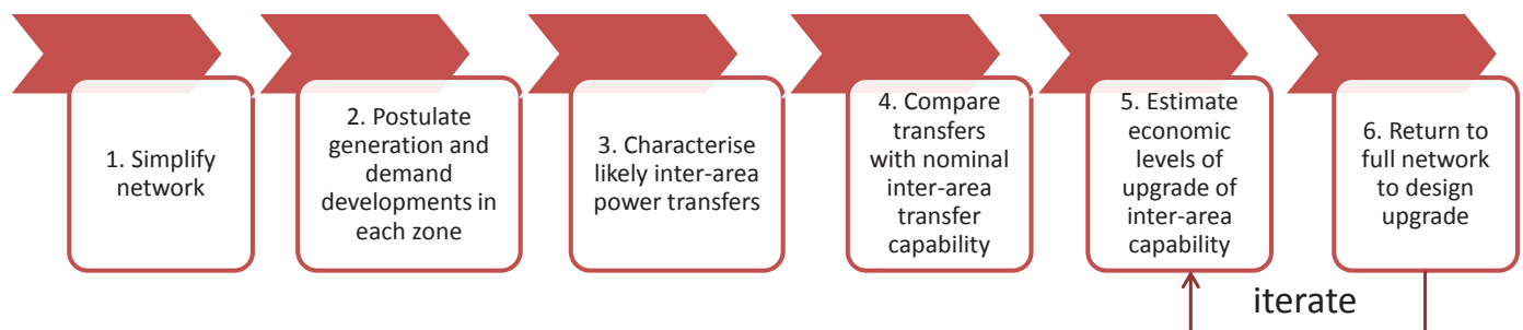
Figure C.1: A proposed iterative approach to transmission planning that allows many scenarios to be studied.
