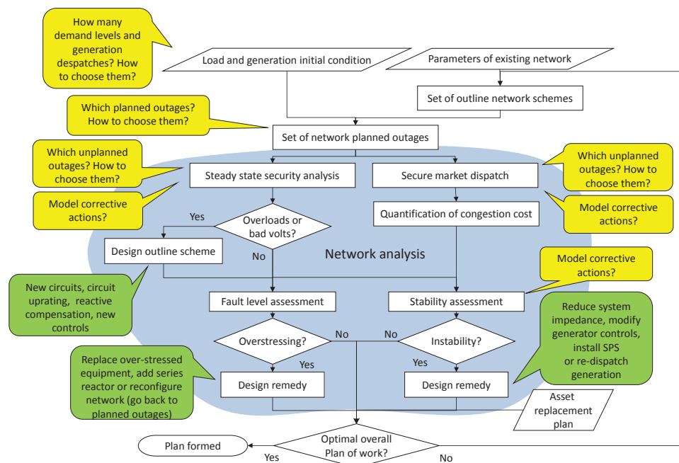
Figure C.2: Detailed study of the facilitation of a given increase in net transfer capacity.
