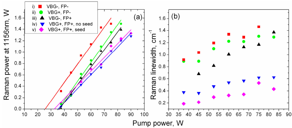
Fig. 3. Raman laser output power (a) and linewidths of the Raman laser emission (b) as functions of diode incident pump power for different cavity configurations.
