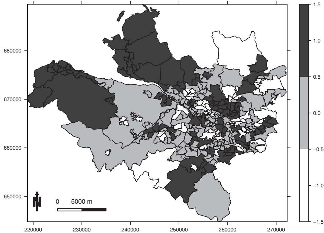
Figure 2. A map showing the piecwise constant mean function (with possible values \{-1, 0, 1\} ) for the random effects that generate localized spatial correlation in the simulation study.
