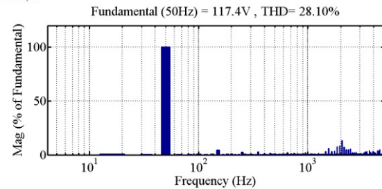
(b) Spectrum of the output voltage
