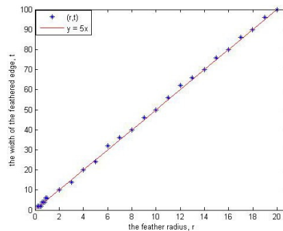
Fig.5. The relationship between t and r
