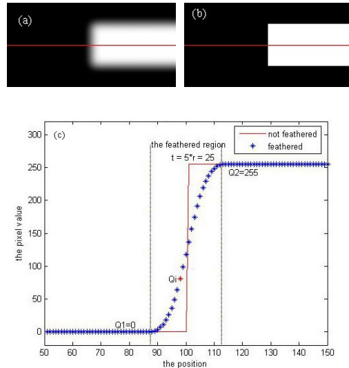
Fig.4. Feathered image (a) and un-feathered edge (b). Profile of the red line in (c) to show the difference between the feathered edge and un-feathered edge.
