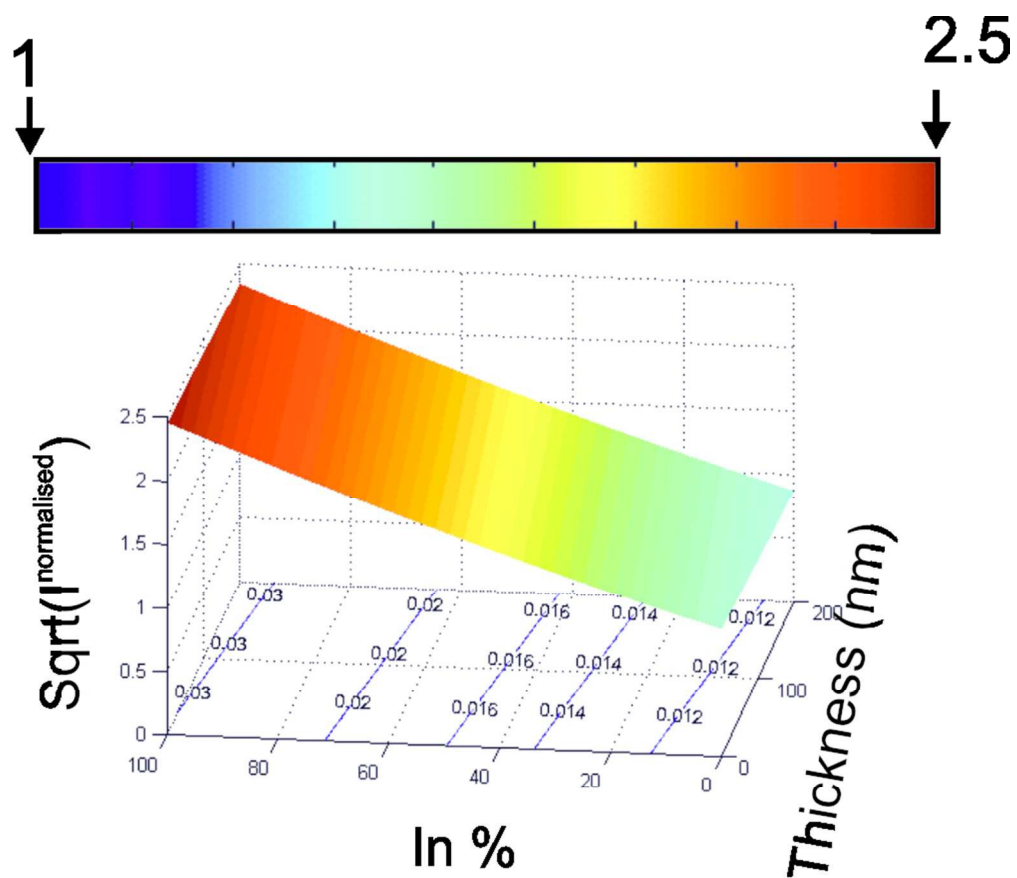
Figure 3) Plot of \sqrt{\left(\frac{Z_{\text{eff}}(\text{InGaN})^2 \cdot (Q_{\text{InGaN}} - 1/2) \cdot (t_{\text{Q}}_{\text{InGaN}})^2}{Z_{\text{eff}}(\text{GaN})^2 \cdot (Q_{\text{GaN}} - 1/2) \cdot t_{\text{Q}}(\text{GaN})^2}\right)} versus x in an [\text{In}]_x [\text{Ga}]_{(1-x)} \text{N} alloy and specimen thickness t from 0 to 200nm and the linear fit. The contour shows the residue to the linear fit. 85x73mm (300 x 300 DPI)
