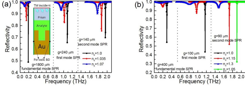
FIG. 5 The reflectivity spectra of different mode SPR sensing at a different incident angle. (a) for internal incident angle \theta_{\text{int}} = 45^\circ ; (b) for internal incident angle \theta_{\text{int}} = 60^\circ . The dot lines in figure are for eye-guide to distinguish the different mode SPR. Note the minimal detection refractive index for the second mode-base sensing of large angle input is n_d = 1.05 . The inset in panel (a) is the simulation schematic.
