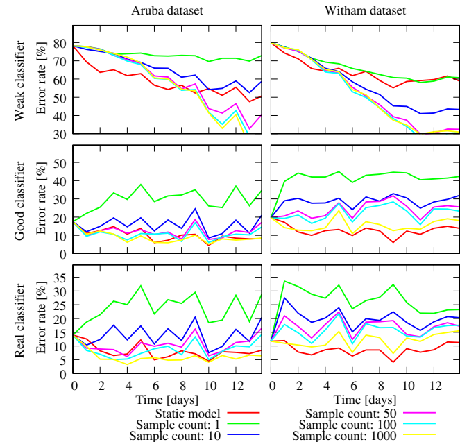
Figure 8. Impact of the number of samples used for prior estimation on the performance of the Adaptive Interval Models. Best viewed in color.
