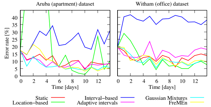
Figure 11. The impact of various spatial and temporal priors on the activity recognition error over time - good classifier with 20% classification error.
