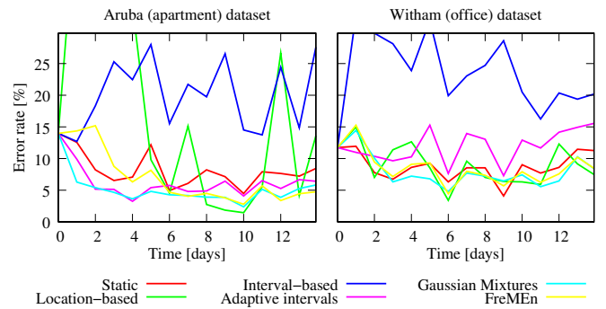
Figure 12. The impact of various spatial and temporal priors on the activity recognition error over time - real classifiers with \sim 13\% classification error.
