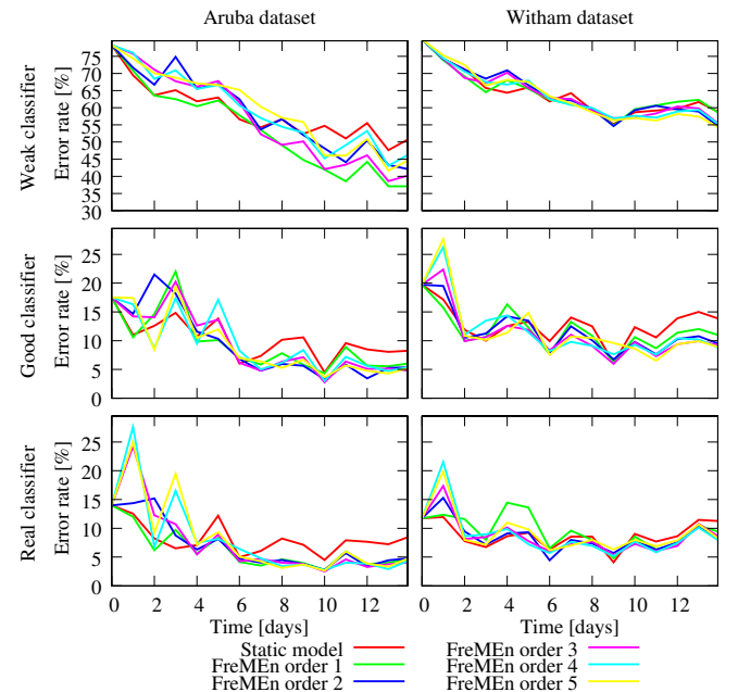
Figure 5. Impact of the number of modelled periodical processes on the FreMEn model. Best viewed in color.
