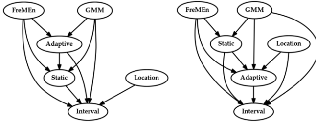
Figure 9. Comparative performance of the examined methods on the Aruba (left) and the Witham (right) dataset. An arrow from A to B indicates that method A has a significantly lower classification error than method B.
