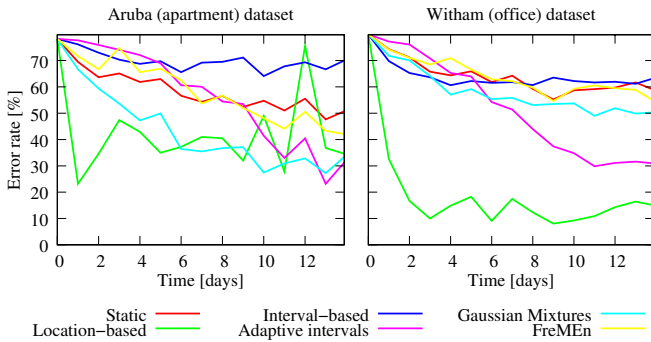
Figure 10. The impact of various spatial and temporal priors on the activity recognition error over time - weak classifier with 80% classification error.
