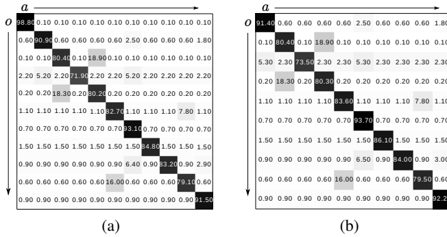
Figure 4. Confusion matrices which characterize the p(o|a) of the ‘real’ classifiers for the Aruba(a) and Witham(b) datasets.
