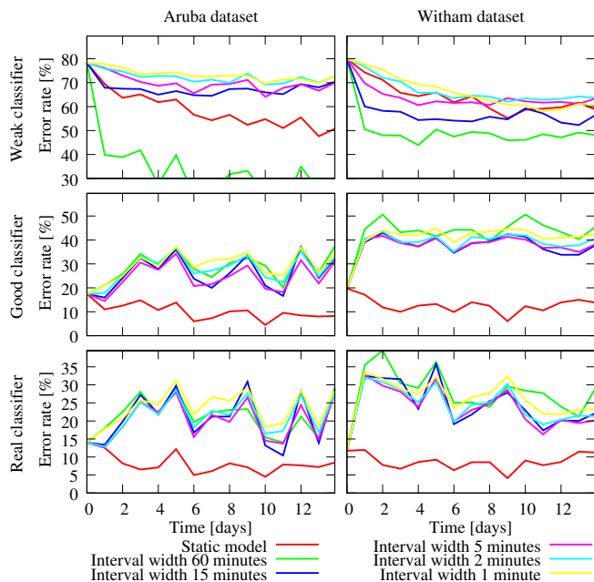
Figure 7. Impact of the interval width on the performance of the Interval models. Best viewed in color.
