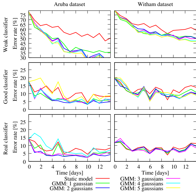
Figure 6. Impact of the number of Gaussians included on the performance of the Gaussian Mixtures. Best viewed in color.
