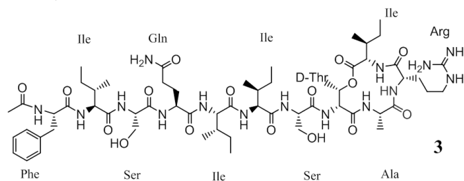
Figure 4: Structure of analogue 3
