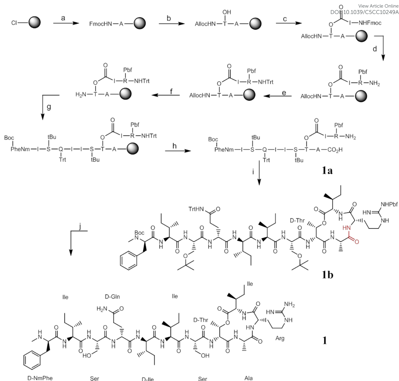
Figure 3: Total synthesis of analogue 1 starting from 2-Chlorotritylchloride resin: a. 4 eq. Fmoc-Ala-OH/8 eq. DIPEA in DCM, 3h. b. 20% piperidine in DMF followed by 3 eq. AllocHN-D-Thr-OH, 3 eq. HATU/6 eq. DIPEA. c. 10 eq. Fmoc-Ile-OH, 10 eq. DIC, 5 mol% DMAP in DCM, 2h followed by capping with Ac 2 O/DIPEA 10% in DMF, 20% piperidine in DMF. d. 4 eq. Fmoc-Arg(Pbf)-OH, 4 eq. HATU/8 eq. DIPEA in DMF, 1h followed by 20% piperidine in DMF. e. 10 eq. Trt-Cl, 15% Et 3 N in DCM, 1h. f. [Pd(PPh 3 ) 4 ] 0 (0.2 eq.) + 24 eq. PhSiH 3 in DCM, 2 x 1 h. g. Fmoc/Boc-AA(PG)-OH (AA = amino acid, PG = protecting group), HATU/DIPEA followed by 20% piperidine in DMF. h. TFA:TIS:DCM = 2:5:93, 2h. i. 1 eq. HATU/10 eq. DIPEA in DMF, 1h, monitored on HPLC. j. TFA:TIS:H 2 O = 95:2.5:2.5, 1h.
