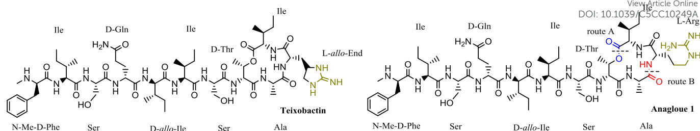
Figure 1a: (left) Structure of teixobactin. Figure 1b: (right) Structure of the teixobactin analogue 1 showing the bonds to be cleaved for the synthesis routes A (in blue) and B (in red) and the structural differences (in green)
