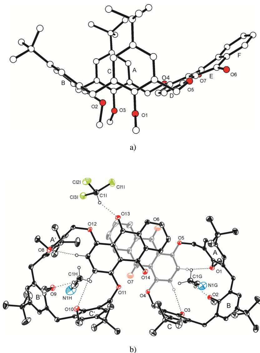
Figure 4. a) Molecular structure of macrocycle 1 in the 2:2:1 inclusion with acetonitrile and chloroform ( 1a ). Only host molecule 1 is displayed; all guest molecules and hydrogen atoms have been omitted for clarity. The disorder of the two
