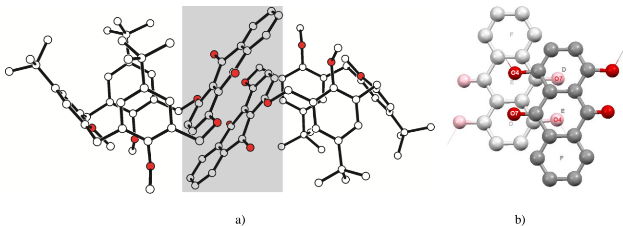
Figure 7. a) Dimer formation in the packing of 2 in its 1:3 acetonitrile inclusion compound ( 2a ). Guest molecules and hydrogen atoms are left out for clarity. b) The two paired anthraquinone units in 2a resemble a charge-transfer complex.
