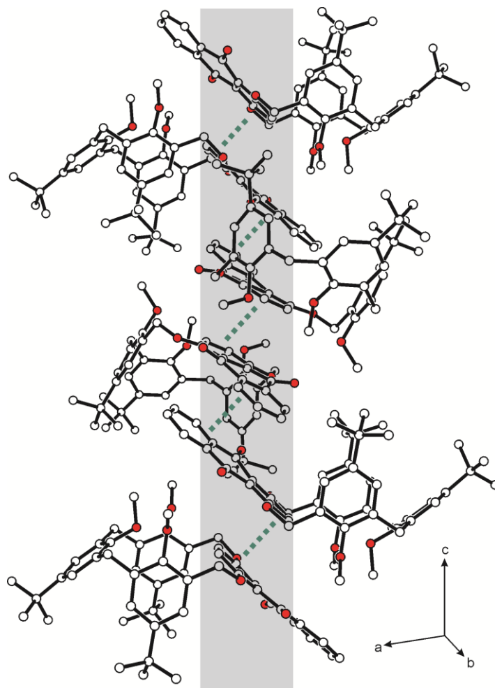
Figure 5. Packing details in the inclusion compound 1a . The characteristic stacking of the anthraquinone moieties is highlighted in grey. Disordered tert -butyl groups, guest molecules and hydrogen atoms are left out for clarity.
