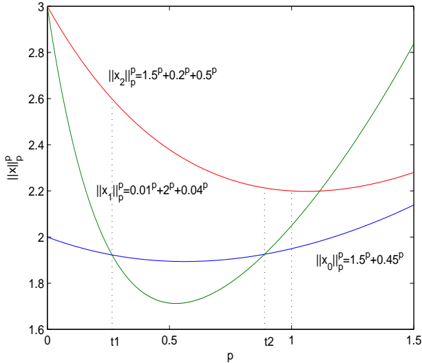
Fig. 2. The optimal solution to l_p -minimization varies with decreasing p .
