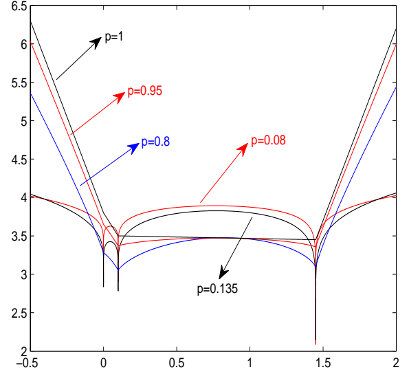
Fig. 4. Behaviors of the l_p -norms as the functions of t for p = 0.08, 0.135, 0.8, 0.95 and 1 , respectively.
