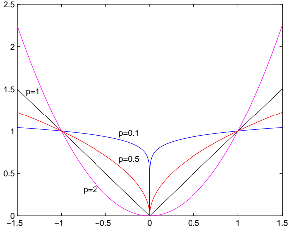
Fig. 1. The behavior of l_p -norm for various values of p . See, e.g. [3, p.38]
