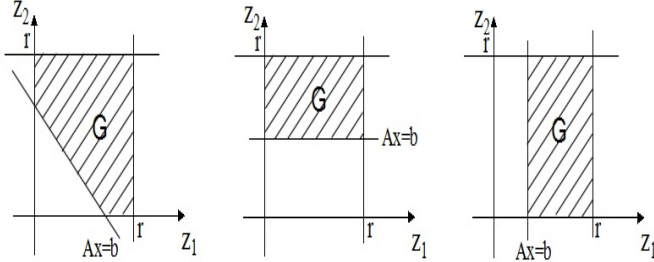
Fig. 3. Shapes of the polytope G(r) defined as in (3) in the plane.
