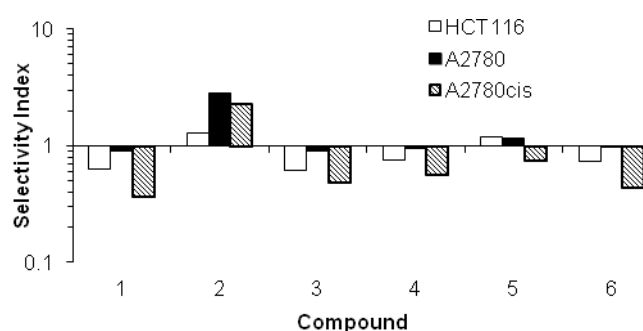
Figure 3 Show the selectivity index defined as the IC 50 in ARPE-19 divided by IC 50 relevant cancerous cells. An SR = 1 indicates equitoxic potency against tumour and normal cells. An SR > 1 indicates preferential selectivity for tumour cells compared to normal cells. An RF < 1 indicates poor selectivity (greater cytotoxicity towards ARPE cells compared to normal cells)
