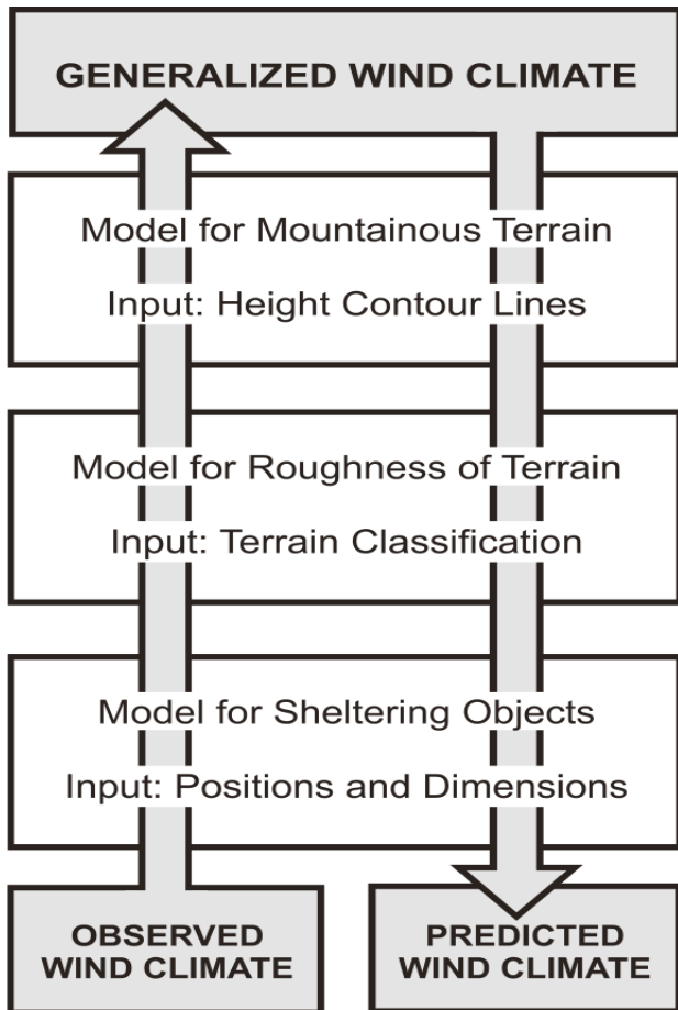
Figure 3.1. Wind Atlas Methodology (adapted from Troen and Petersen, 1989)
