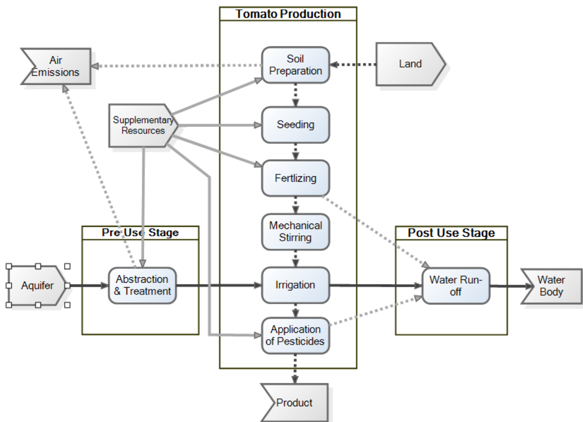
Figure 2. Stages of water value chain and tomato crop
