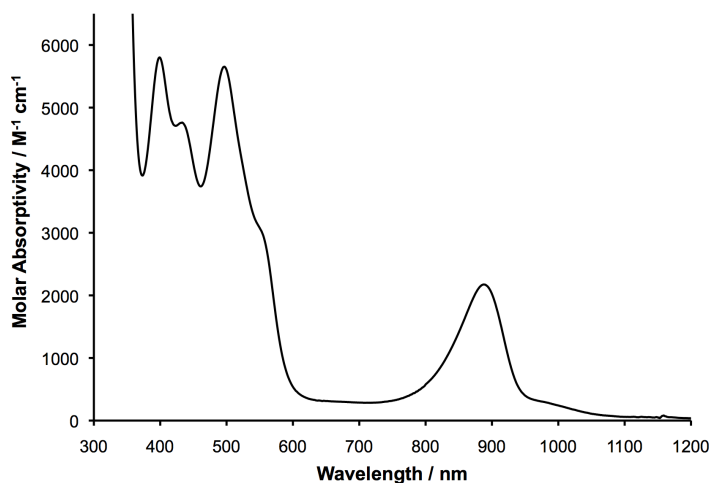
Figure 5. Electronic absorption spectrum of a 0.34 mmol solution of \text{Ru}_2(\text{dmof})_4 recorded in dichloromethane.
