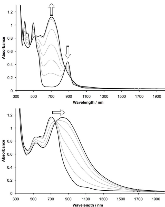
Figure 6. UV/vis/NIR spectroelectrochemical study of a 1.3 mmol solution of \text{Ru}_2(\text{dmof})_4 in 0.1 M n\text{Bu}_4\text{NPF}_6 / \text{CH}_2\text{Cl}_2 at room temperature. Spectral changes associated with the \text{Ru}_2^{4+} \rightarrow \text{Ru}_2^{5+} oxidation are shown on top, and those associated with the \text{Ru}_2^{5+} \rightarrow \text{Ru}_2^{6+} oxidation on the bottom.
