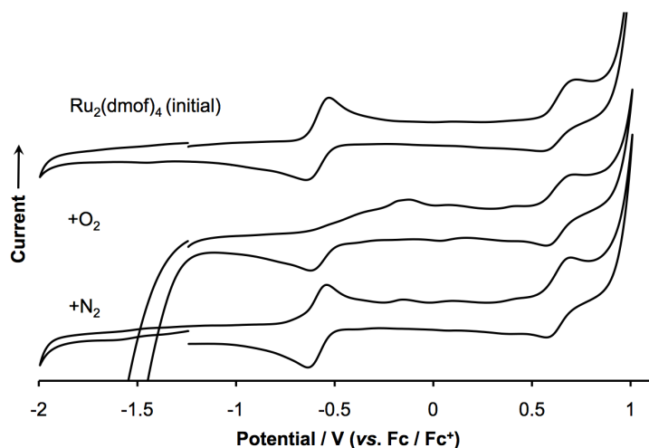
Figure 8. Cyclic voltammogram (0.1M n\text{Bu}_4\text{NPF}_6 / \text{CH}_2\text{Cl}_2 ) of \text{Ru}_2(\text{dmof})_4 before (top) and after (middle) exposure of the cell to \text{O}_2 gas. The bottom voltammogram was obtained by bubbling \text{N}_2 through the cell after the addition of \text{O}_2 .
