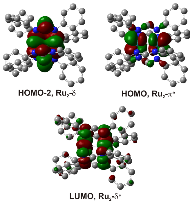
Figure 3. Selected MO plots for Ru 2 (C 6 H 5 N{CH}NC 6 H 5 ) 4 (0.02 isosurface value).
