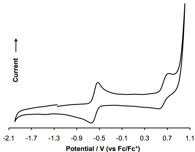
Figure 4. Cyclic voltammogram of \text{Ru}_2(\text{dmof})_4 recorded in a 0.1 M {}^t\text{Bu}_4\text{PF}_6 / \text{CH}_2\text{Cl}_2 solution at room temperature.
