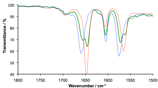
Figure 2. IR spectra of 20 mM solutions [\text{I}]_2 (red), [\text{I}]_2^{2+} (green) and [\text{I}]_2^{2+} (blue) recorded in 0.1 M \text{NBu}_4\text{PF}_6 / \text{CH}_2\text{Cl}_2 at -30^\circ\text{C} using a spectroelectrochemical cell.
