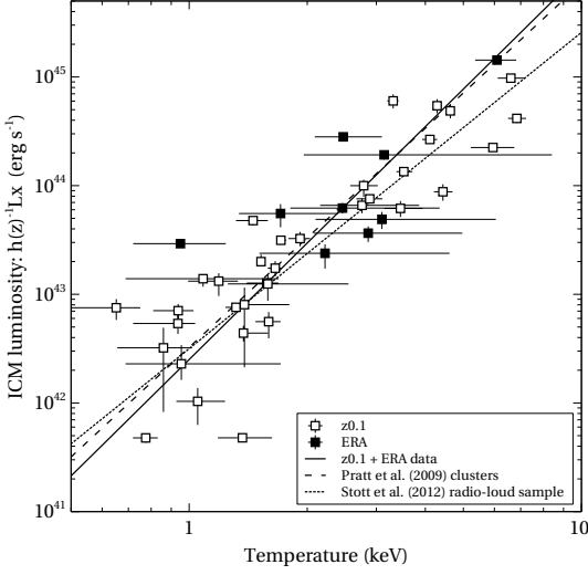
Figure 11. ICM luminosity vs temperature for the temperatures obtained by spectral analysis. Empty squares denote the z0.1 sample and filled squares denote the ERA sample. The solid line shows the L_X - T_X relationship from the combined samples, and the dashed line shows Pratt et al. (2009)’s L_X - T_X relation for clusters. Also shown is the relation from Stott et al. (2012) for their sub-sample of clusters containing radio galaxies (dotted line).
