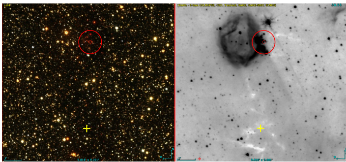
Fig. 5: Area of cluster candidate La Serena 208. Left panel: VVV color-composite image following the same scheme as in Figure 1. Right panel: Spitzer/GLIMPSE 8\mu\text{m} . The cluster candidate is marked with a small red circle, and the dark cloud SDC G321.336 – 0.373 with a small yellow plus sign. The field of view of each panel is about 9.8 \times 9.0 arcmin.
