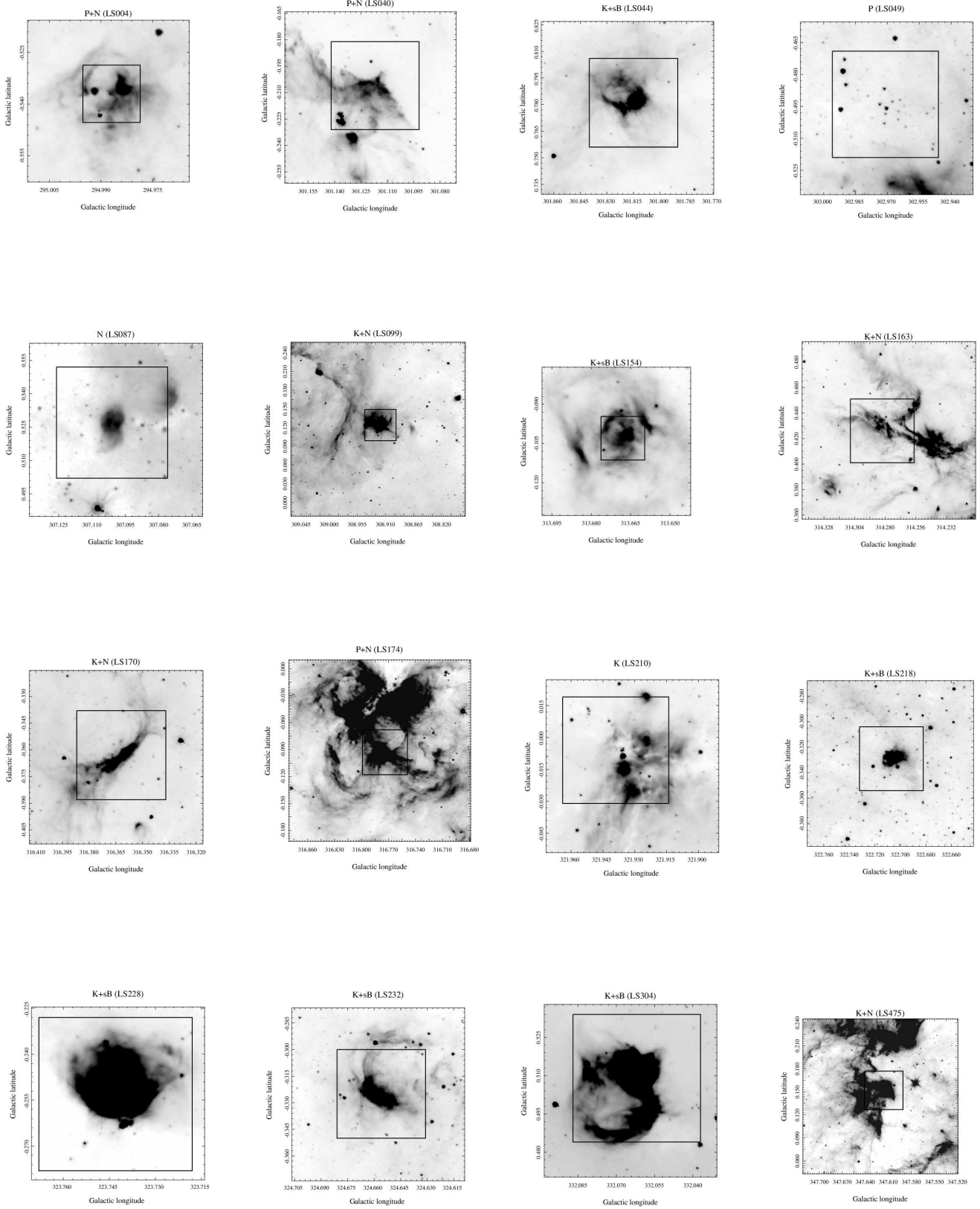
Fig. 9: Examples of different cluster morphologies based on images in the 8 \mu\text{m} band obtained with the Infrared Array Camera (IRAC) on board the Spitzer Space Telescope. Boxes inside each panel correspond to the cluster candidate charts showed in Figure 1.
