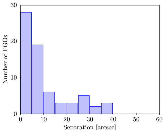
Fig. 8: Histogram of the number of EGO and outflow candidates associated with the new VVV – La Serena star cluster candidates.
