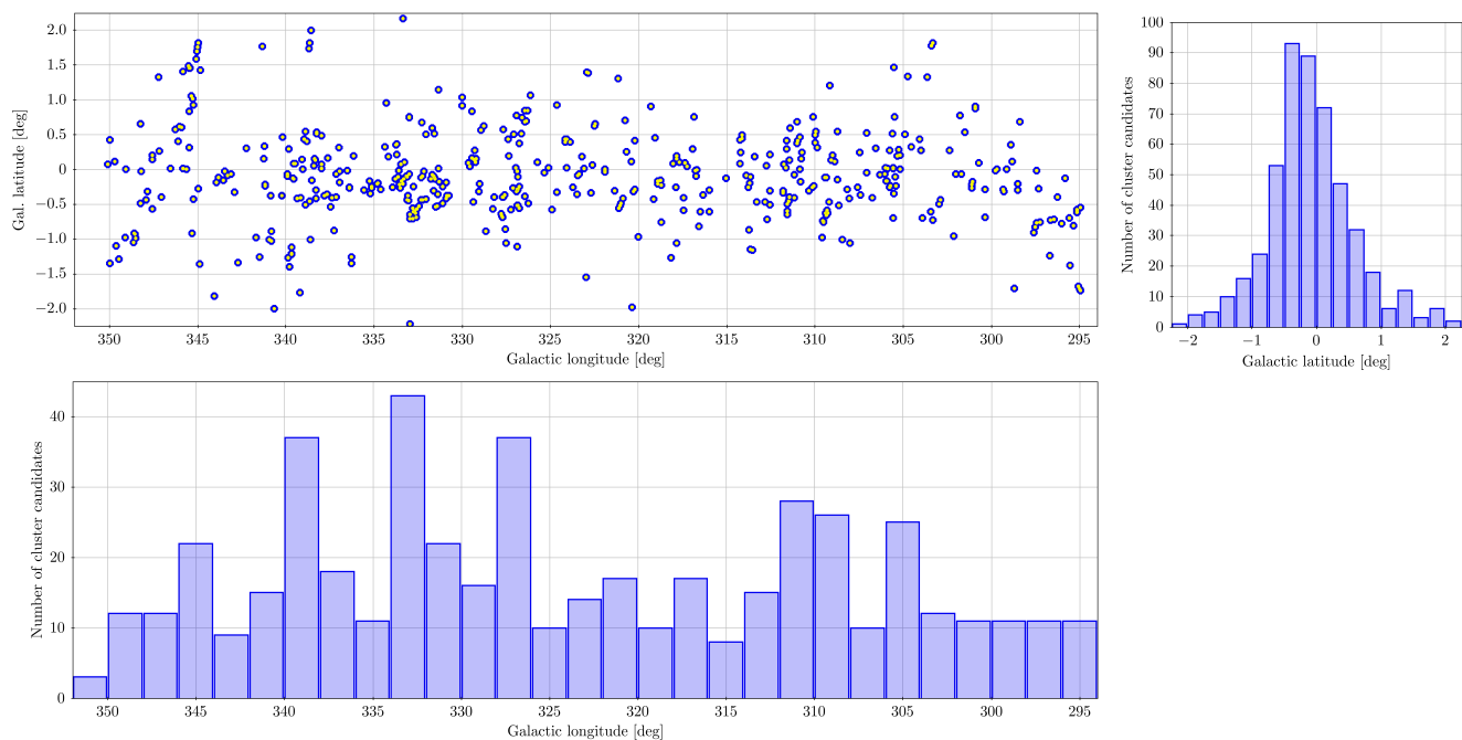
Fig. 2: Angular distribution of the newly discovered La Serena star cluster candidates in the Galactic plane (upper left panel). Also, the histograms of the distributions of clusters in Galactic latitude (upper right panel) and Galactic longitude (lower panel).
