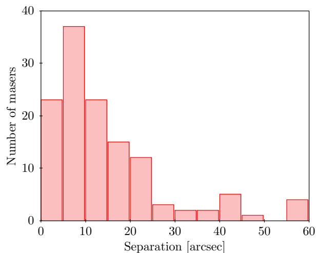
Fig. 6: Histogram of the number of masers associated with the new VVV – La Serena star cluster candidates.
