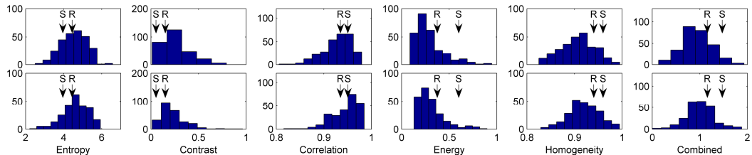
Figure 2. Frequency distributions of statistical features of 2D patterns from cirrus (top row) and mixed phase (lower row) flights. Arrows show values for the smooth (S) and moderately rough (R) ice analogues from Fig. 1. The "combined" feature is (energy + homogeneity - contrast). Note that all but entropy and contrast are anticorrelated with roughness.
