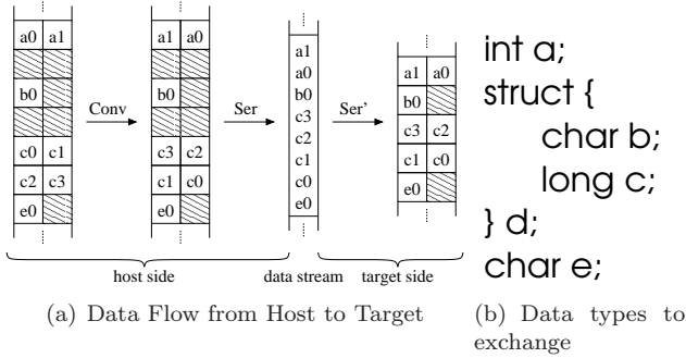
Figure 4. Example of Data Exchange: Sending Data from Host to Target
