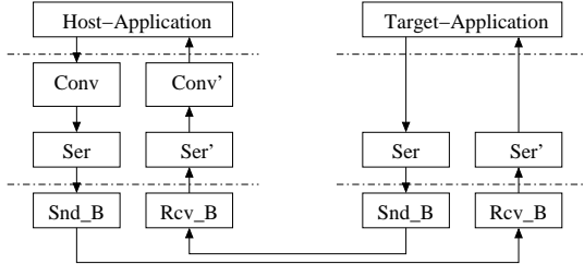
Figure 3. “Host-Makes-Right” Method
