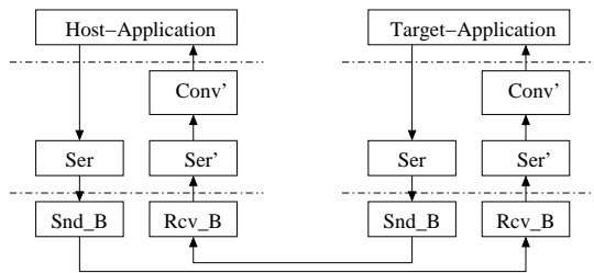
Figure 1. “Receiver-Makes-Right” Method
