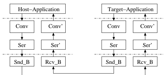
Figure 2. “Symmetric Conversion” Method
