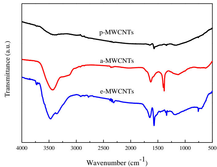
Fig. 3 FTIR spectra of p-MWCNTs, a-MWCNTs and e-MWCNTs.
