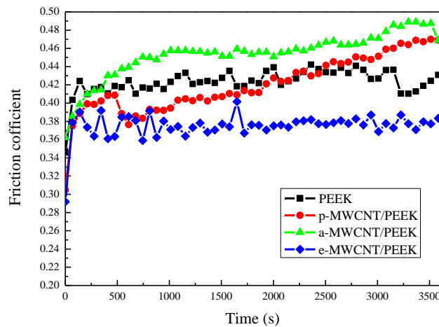
Fig. 7 Friction coefficient versus time of MWCNT/PEEK composites (4% MWCNTs) at the load of 3.929 N and sliding velocity of 0.0295 m/s.
