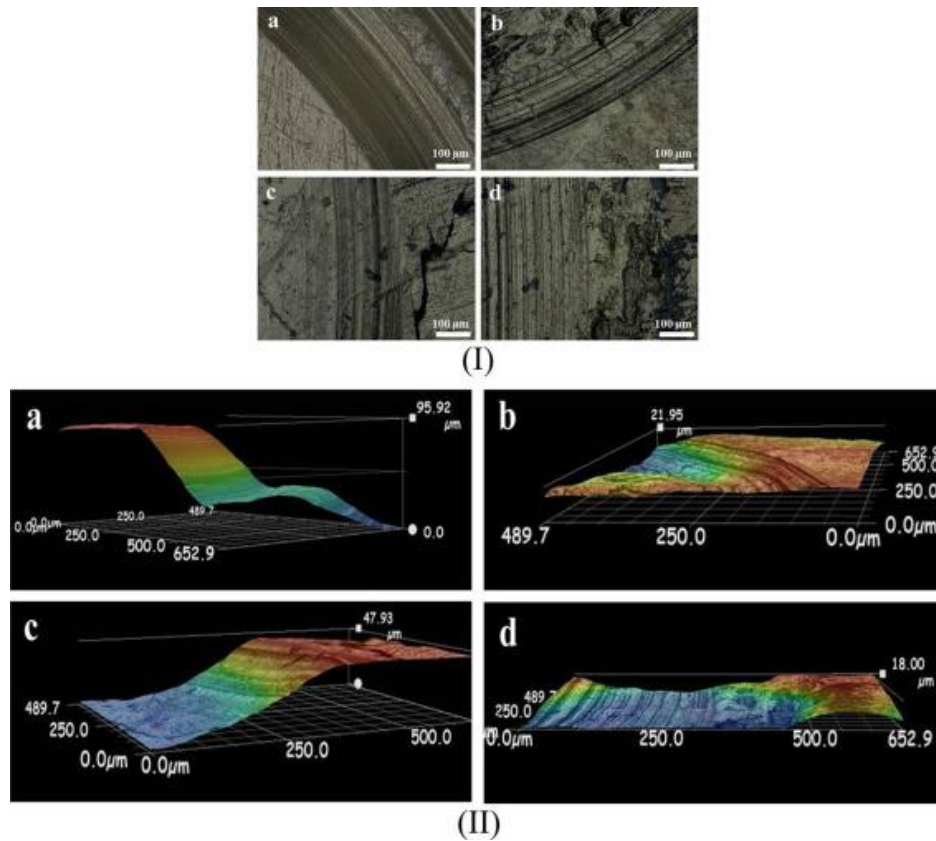
Fig. 8 The morphology of the wear surfaces (I) and the scratching depth (II) of pure PEEK and MWCNT/PEEK composites: (a) pure PEEK, (b) p-MWCNT/PEEK, (c) a-MWCNT/PEEK and (d) e-MWCNT/PEEK.
