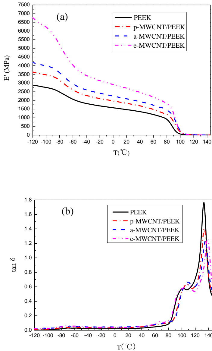
Fig. 6 DMA spectra of pure PEEK and different types of MWCNT/PEEK composites (4% MWCNTs) at a frequency of 1 Hz: (a) Storage modulus E' versus temperature; (b) \tan \delta versus temperature.
