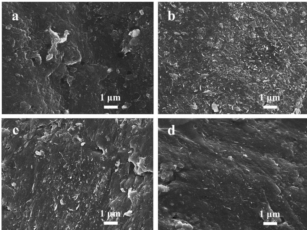
Fig. 9 Typical wear scars of pure PEEK and MWCNT/PEEK composites: (a) pure PEEK, (b) p-MWCNT/PEEK, (c) a-MWCNT/PEEK, (d) e-MWCNT/PEEK.
