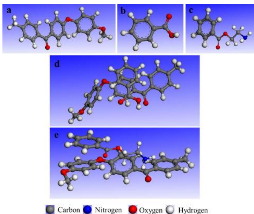
Fig. 5 Optimized structures of finite PEEK and MWCNT/PEEK composites: (a) PEEK, (b) a-MWCNTs, (c) e-MWCNTs, (d) a-MWCNT/PEEK and (e) e-MWCNT/PEEK.
