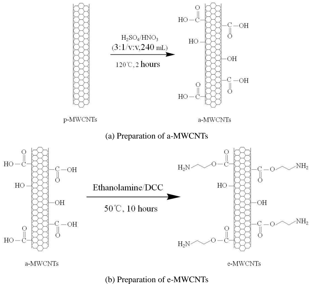
Fig.1 The schematic views of principles in surface modification of MWCNTs: preparation of (a)a-MWCNTs and (b) e-MWCNTs.
