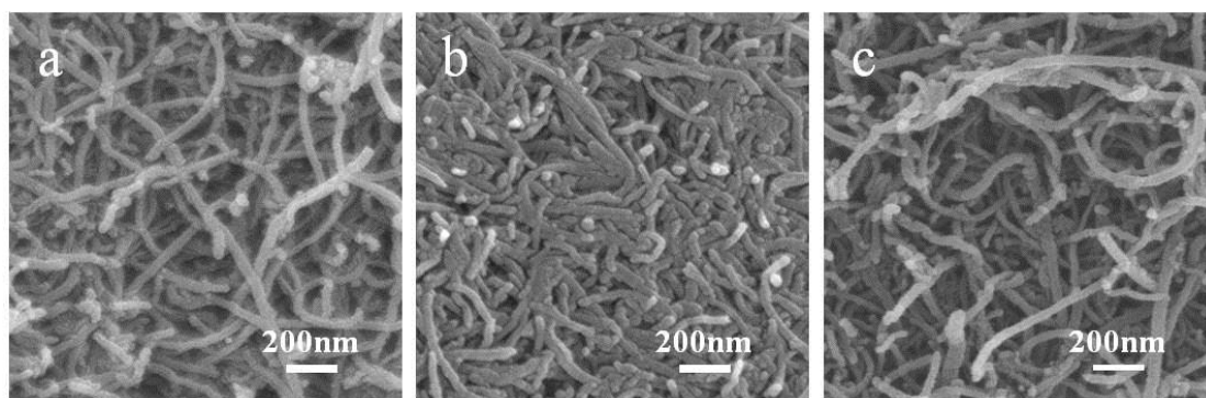
Fig. 2 SEM observations of different MWCNTs: (a) p-MWCNTs, (b) a-MWCNTs, (c) e-MWCNTs.
