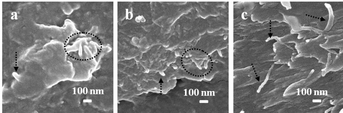
Fig. 4 SEM observations of different MWCNT/PEEK composites: (a) p-MWCNT/PEEK, (b) a-MWCNT/PEEK, (c) e-MWCNT/PEEK.
