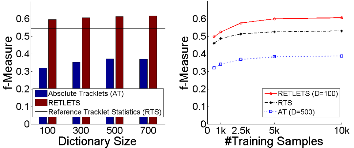
Figure 7.7: Recognition results using Reference Tracklet Statistics, Absolute Tracklets and RETLETS with variation in dictionary size and number of training samples. Note that as Reference Tracklet Statistics are not histograms their performance is constant across dictionary sizes (represented as a horizontal line in the Figure on the left).
