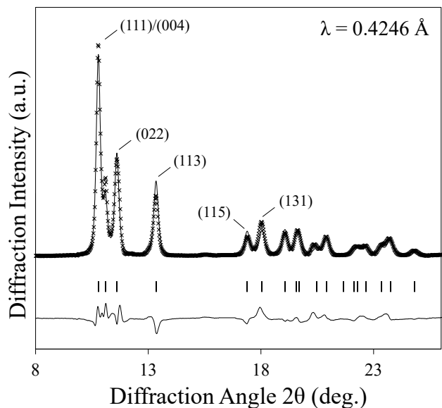
FIG. 2. Rietveld refinement of the oF8 structure to a diffraction profile from Nd at 97 GPa, showing the observed (crosses) and calculated (line) diffraction patterns, and the difference profile ( R_P = 1.8\% , R_{WP} = 2.5\% , goodness of fit (GoF) = 0.46, R(F^2) = 6.1\% ). The first six peaks of the oF8 phase are labelled with their Miller indices.
