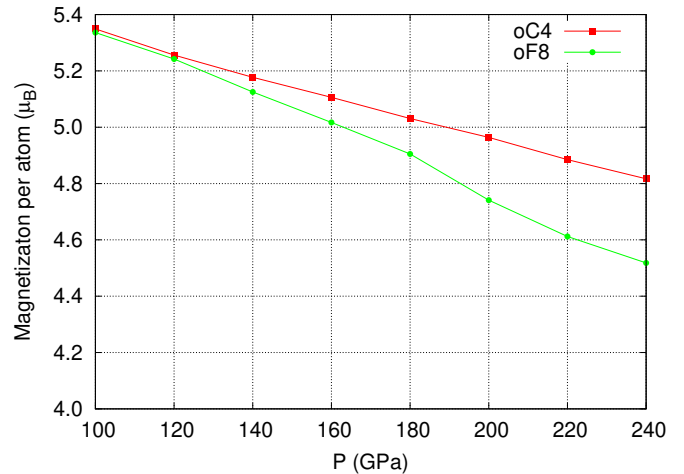
FIG. 12. The calculated magnetisation, in \mu_B/\text{atom} , of the oC4 and oF8 phases of Sm over the pressure range from 100 to 240 GPa. In contrast to the behaviour seen in Nd, the magnetisation, although decreases, is non-zero in both phases at all pressures.
