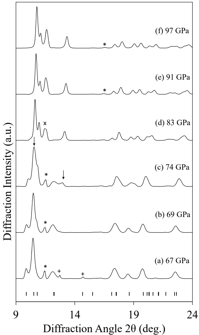
FIG. 1. Diffraction profiles collected from Nd on pressure increase to 97 GPa. The data were collected from the same sample at DLS using a wavelength \lambda = 0.4246 \text{ \AA} . Tick marks beneath profile (a) mark the calculated peak positions in the hP3 phase at this pressure. The peaks marked with asterisks are from the W gasket, and the peaks marked with a + are from the Cu calibrant. The two arrows in profile (c) mark the first appearance of peaks from the post- hP3 phase. The peak labelled with a ‘x’ in profile (d) is a closely-spaced doublet which includes the (110) peak from the W gasket and a peak from the new phase. Single-phase patterns from the post- hP3 phase are seen in profiles (e) and (f).
